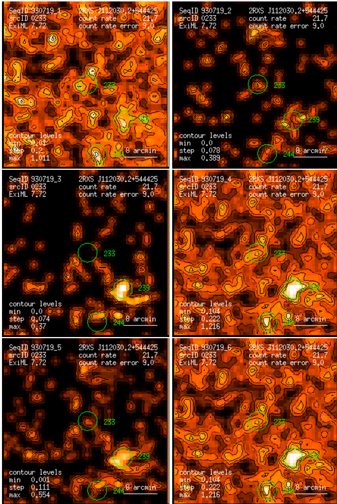
Figure 233: RASS 930719: detection 0233: band rate images, Gaussian filter: (1) PSPC channels 11 – 41, (2) 52 – 90, (3) 91 – 201, (4) 11 – 235, (5) 52 – 201, (6) 11 – 201. Broad band rates in counts/ks. Band rate contour levels in counts/ks/arcmin 2 .
