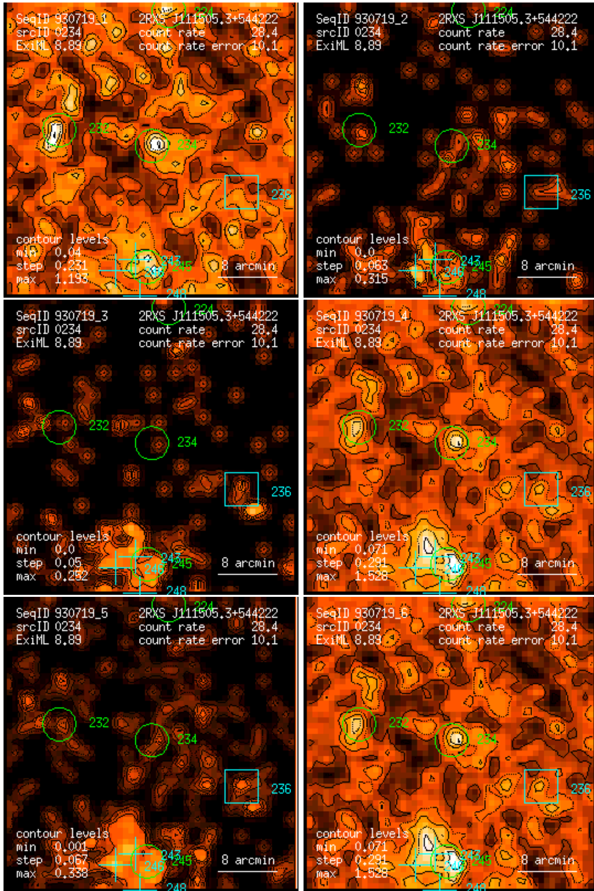
Figure 234: RASS 930719: detection 0234: band rate images, Gaussian filter: (1) PSPC channels 11 – 41, (2) 52 – 90, (3) 91 – 201, (4) 11 – 235, (5) 52 – 201, (6) 11 – 201. Broad band rates in counts/ks. Band rate contour levels in counts/ks/arcmin 2 .
