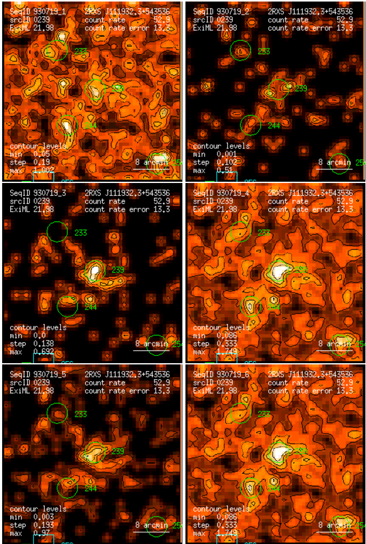
Figure 239: RASS 930719: detection 0239: band rate images, Gaussian filter: (1) PSPC channels 11 – 41, (2) 52 – 90, (3) 91 – 201, (4) 11 – 235, (5) 52 – 201, (6) 11 – 201. Broad band rates in counts/ks. Band rate contour levels in counts/ks/arcmin 2 .
