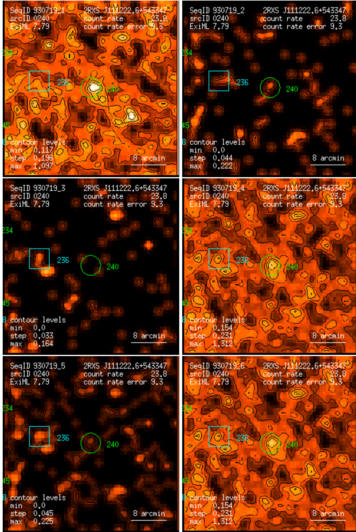
Figure 240: RASS 930719: detection 0240: band rate images, Gaussian filter: (1) PSPC channels 11 – 41, (2) 52 – 90, (3) 91 – 201, (4) 11 – 235, (5) 52 – 201, (6) 11 – 201. Broad band rates in counts/ks. Band rate contour levels in counts/ks/arcmin 2 .
