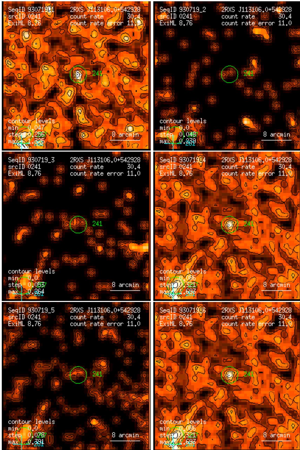
Figure 241: RASS 930719: detection 0241: band rate images, Gaussian filter: (1) PSPC channels 11 – 41, (2) 52 – 90, (3) 91 – 201, (4) 11 – 235, (5) 52 – 201, (6) 11 – 201. Broad band rates in counts/ks. Band rate contour levels in counts/ks/arcmin 2 .
