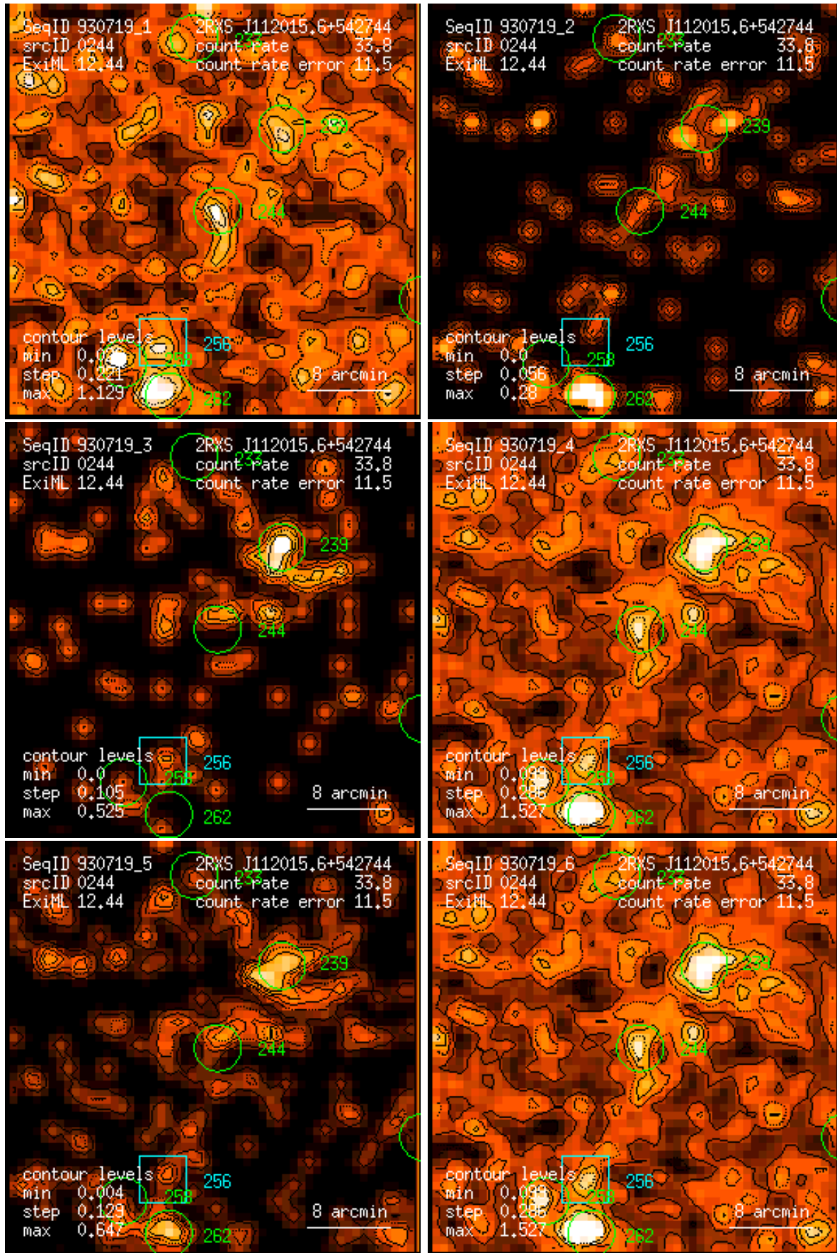
Figure 244: RASS 930719: detection 0244: band rate images, Gaussian filter: (1) PSPC channels 11 – 41, (2) 52 – 90, (3) 91 – 201, (4) 11 – 235, (5) 52 – 201, (6) 11 – 201. Broad band rates in counts/ks. Band rate contour levels in counts/ks/arcmin 2 .
