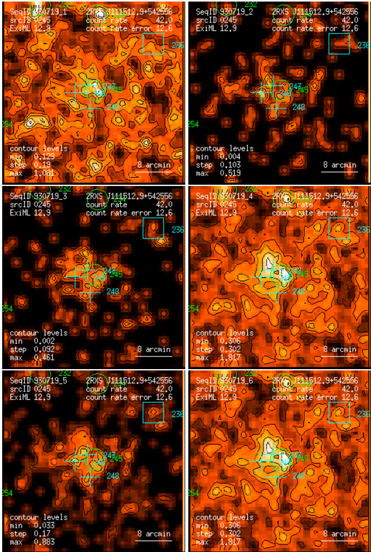
Figure 245: RASS 930719: detection 0245: band rate images, Gaussian filter: (1) PSPC channels 11 – 41, (2) 52 – 90, (3) 91 – 201, (4) 11 – 235, (5) 52 – 201, (6) 11 – 201. Broad band rates in counts/ks. Band rate contour levels in counts/ks/arcmin 2 .
