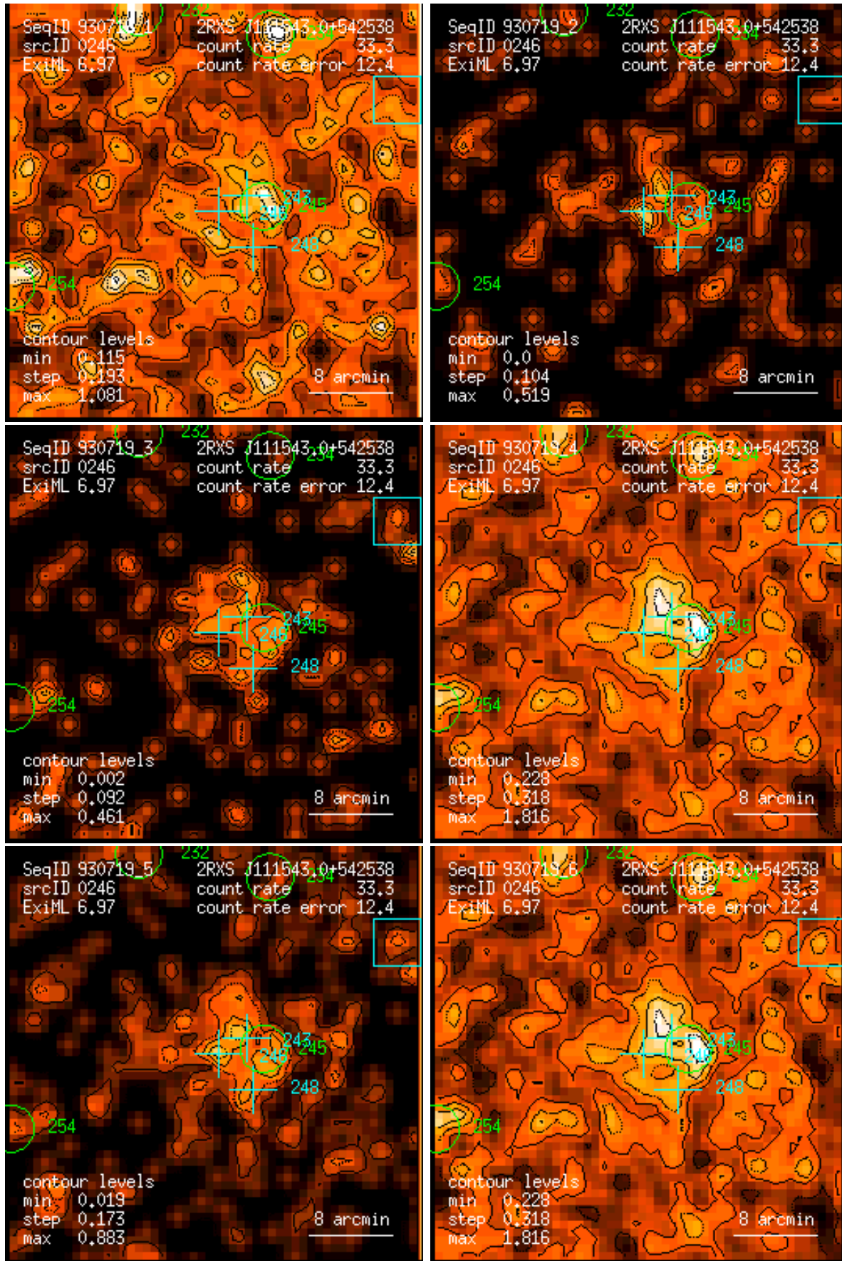
Figure 246: RASS 930719: detection 0246: band rate images, Gaussian filter: (1) PSPC channels 11 – 41, (2) 52 – 90, (3) 91 – 201, (4) 11 – 235, (5) 52 – 201, (6) 11 – 201. Broad band rates in counts/ks. Band rate contour levels in counts/ks/arcmin 2 .
