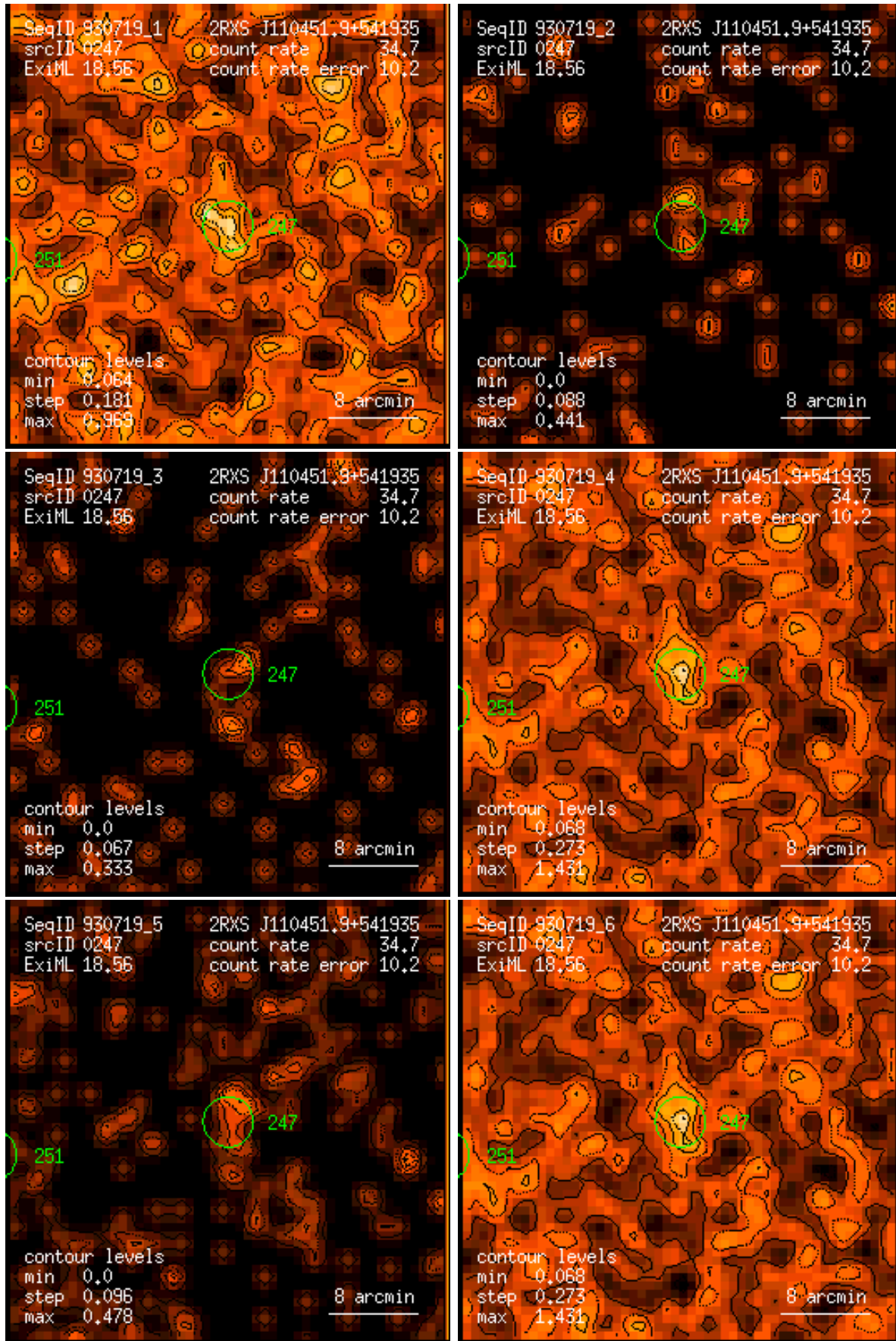
Figure 247: RASS 930719: detection 0247: band rate images, Gaussian filter: (1) PSPC channels 11 – 41, (2) 52 – 90, (3) 91 – 201, (4) 11 – 235, (5) 52 – 201, (6) 11 – 201. Broad band rates in counts/ks. Band rate contour levels in counts/ks/arcmin 2 .
