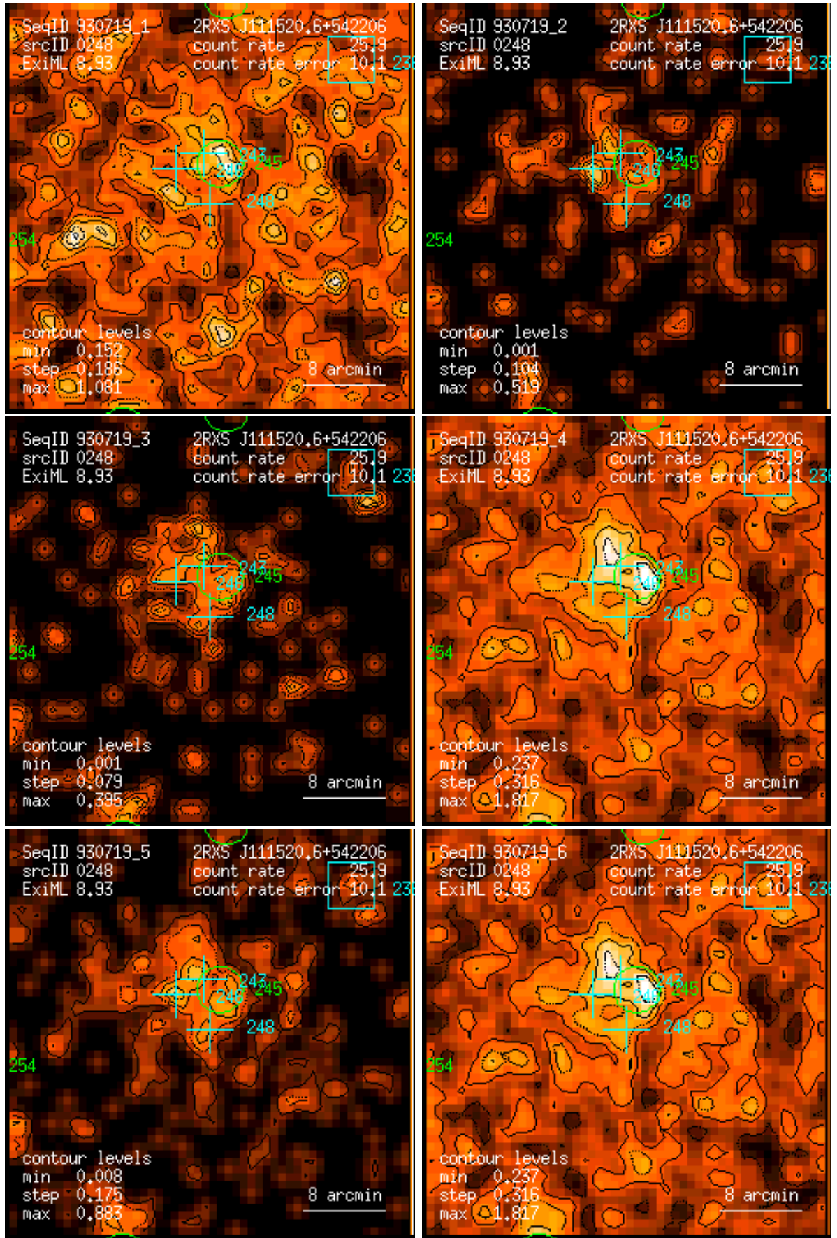
Figure 248: RASS 930719: detection 0248: band rate images, Gaussian filter: (1) PSPC channels 11 – 41, (2) 52 – 90, (3) 91 – 201, (4) 11 – 235, (5) 52 – 201, (6) 11 – 201. Broad band rates in counts/ks. Band rate contour levels in counts/ks/arcmin 2 .
