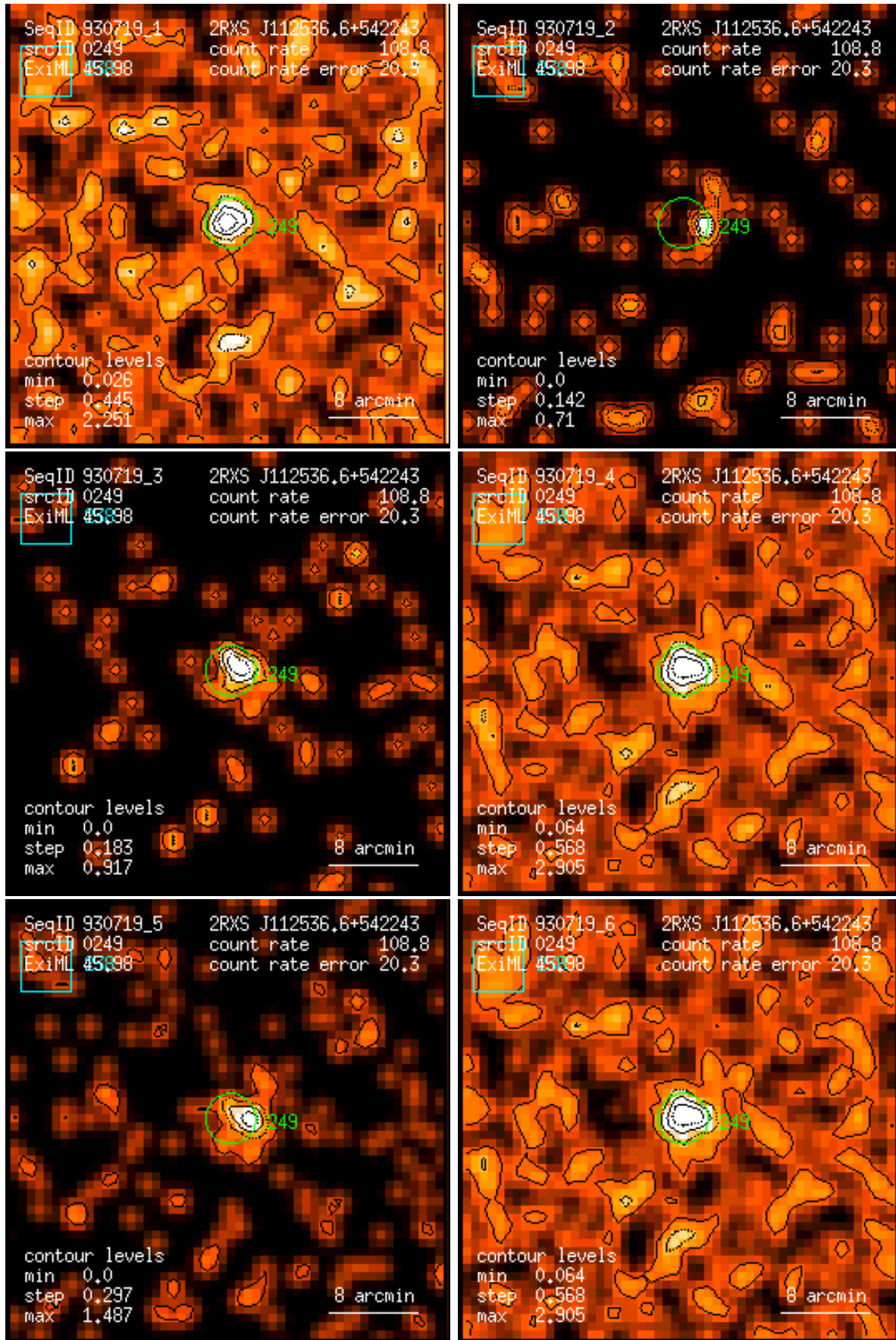
Figure 249: RASS 930719: detection 0249: band rate images, Gaussian filter: (1) PSPC channels 11 – 41, (2) 52 – 90, (3) 91 – 201, (4) 11 – 235, (5) 52 – 201, (6) 11 – 201. Broad band rates in counts/ks. Band rate contour levels in counts/ks/arcmin 2 .
