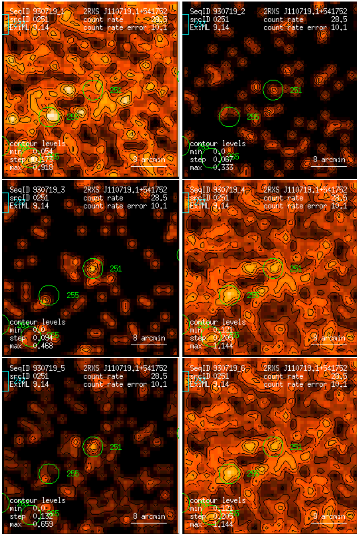
Figure 251: RASS 930719: detection 0251: band rate images, Gaussian filter: (1) PSPC channels 11 – 41, (2) 52 – 90, (3) 91 – 201, (4) 11 – 235, (5) 52 – 201, (6) 11 – 201. Broad band rates in counts/ks. Band rate contour levels in counts/ks/arcmin 2 .
