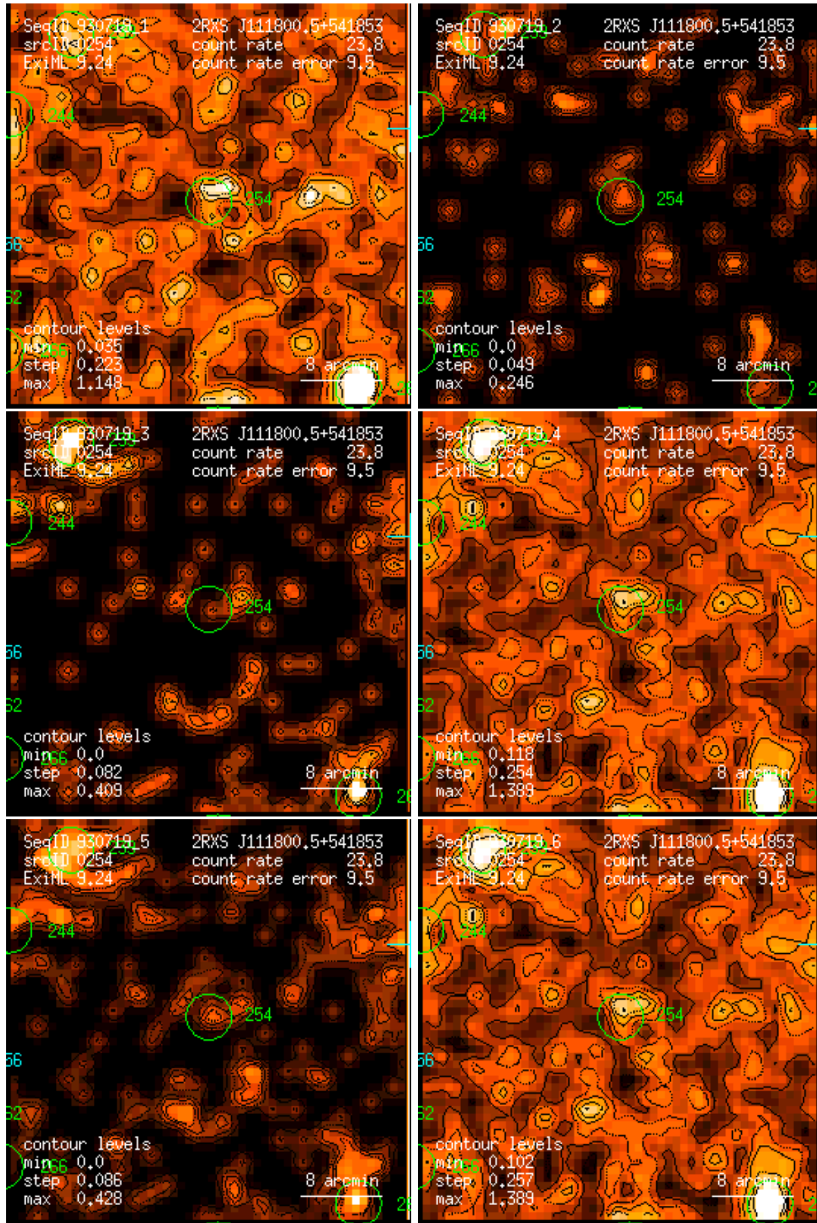
Figure 254: RASS 930719: detection 0254: band rate images, Gaussian filter: (1) PSPC channels 11 – 41, (2) 52 – 90, (3) 91 – 201, (4) 11 – 235, (5) 52 – 201, (6) 11 – 201. Broad band rates in counts/ks. Band rate contour levels in counts/ks/arcmin 2 .
