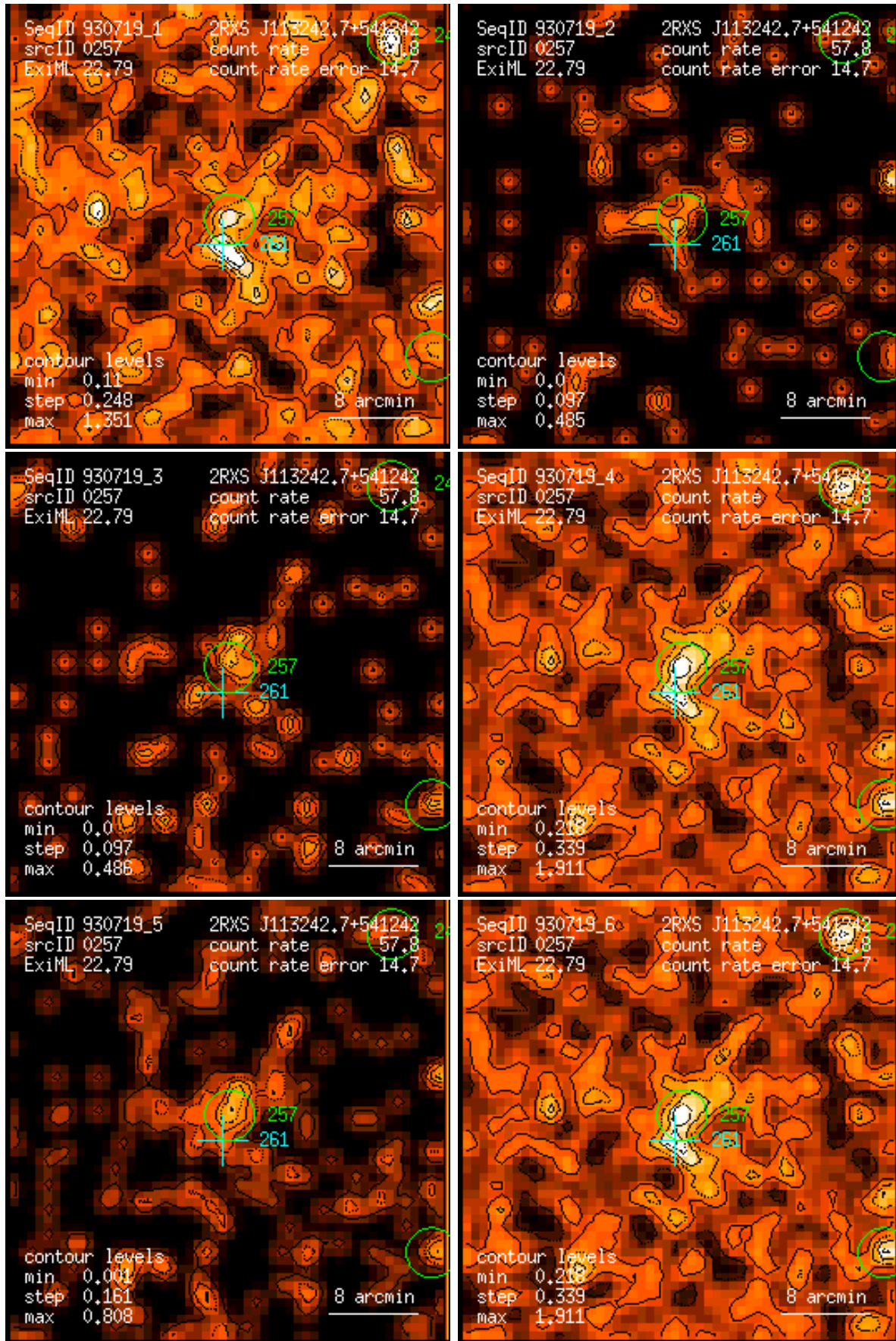
Figure 257: RASS 930719: detection 0257: band rate images, Gaussian filter: (1) PSPC channels 11 – 41, (2) 52 – 90, (3) 91 – 201, (4) 11 – 235, (5) 52 – 201, (6) 11 – 201. Broad band rates in counts/ks. Band rate contour levels in counts/ks/arcmin 2 .
