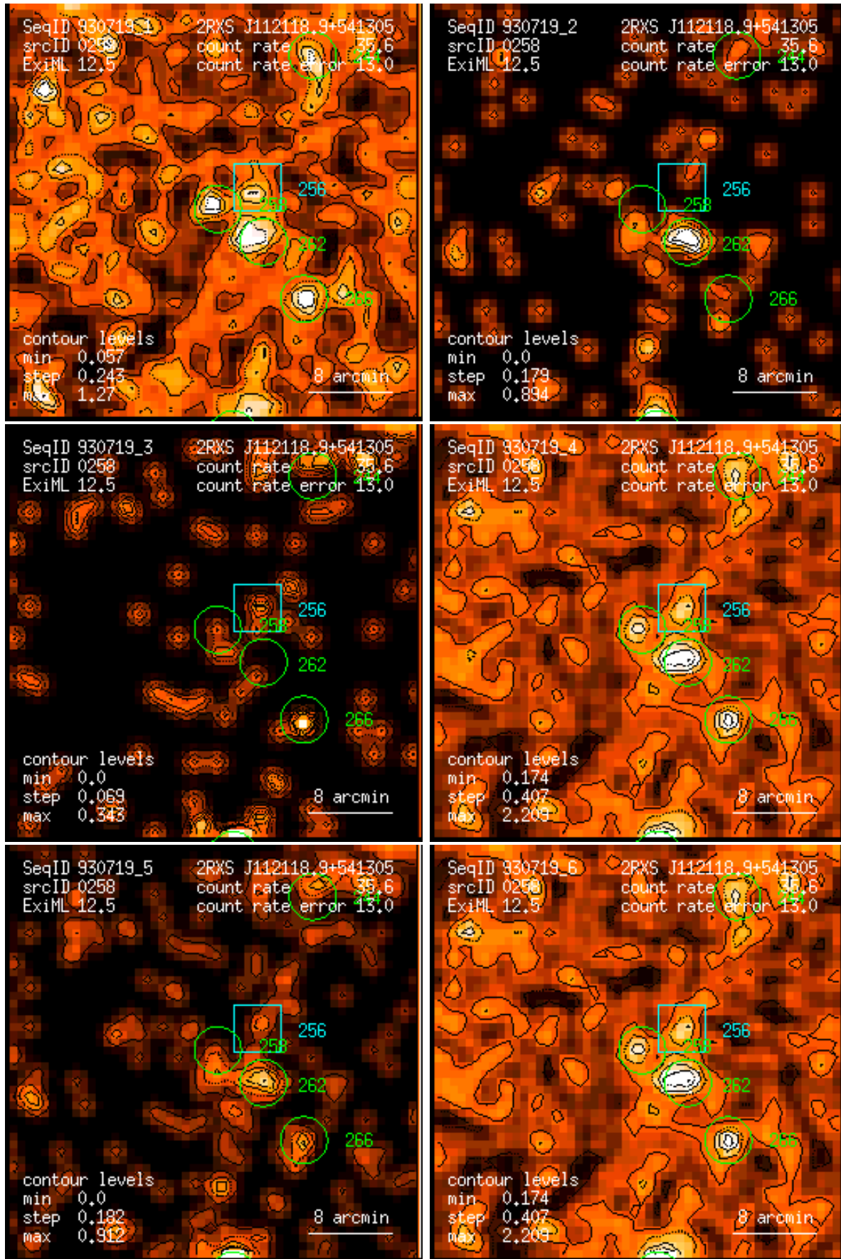
Figure 258: RASS 930719: detection 0258: band rate images, Gaussian filter: (1) PSPC channels 11 – 41, (2) 52 – 90, (3) 91 – 201, (4) 11 – 235, (5) 52 – 201, (6) 11 – 201. Broad band rates in counts/ks. Band rate contour levels in counts/ks/arcmin 2 .
