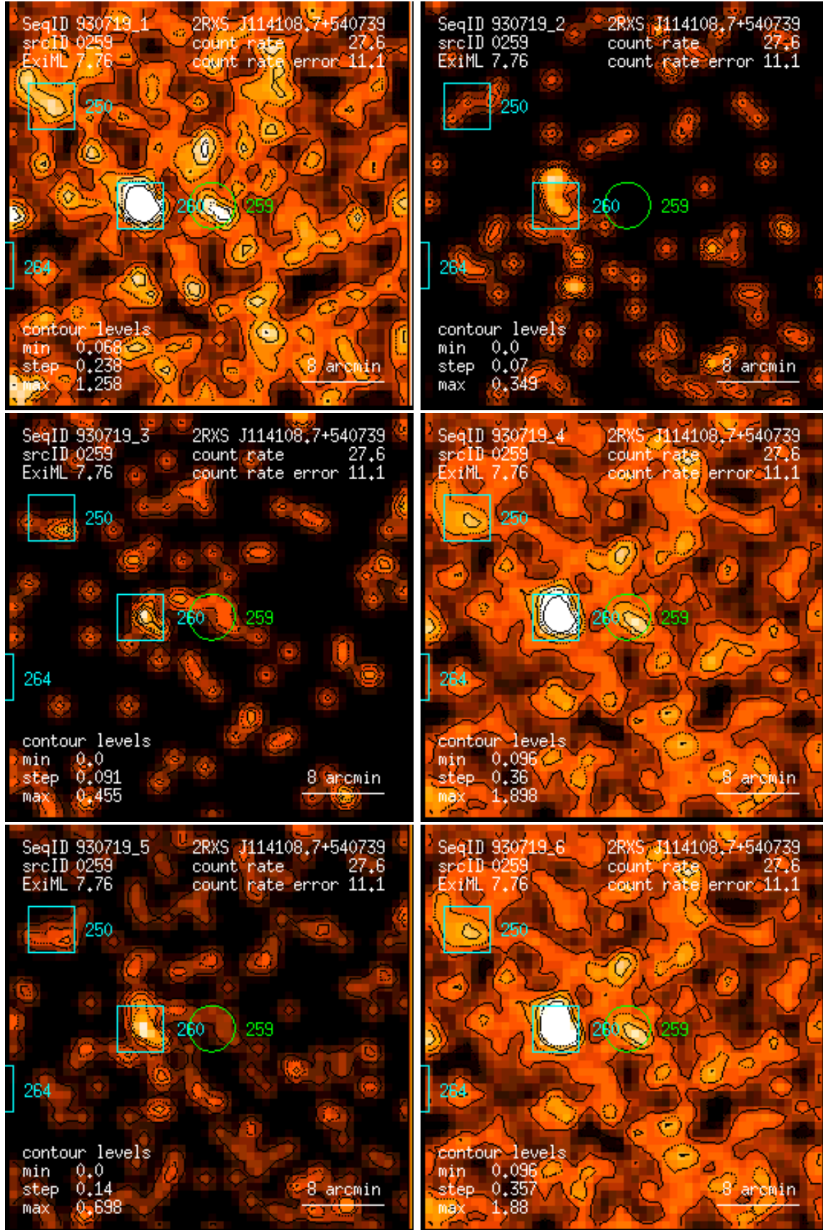
Figure 259: RASS 930719: detection 0259: band rate images, Gaussian filter: (1) PSPC channels 11 – 41, (2) 52 – 90, (3) 91 – 201, (4) 11 – 235, (5) 52 – 201, (6) 11 – 201. Broad band rates in counts/ks. Band rate contour levels in counts/ks/arcmin 2 .
