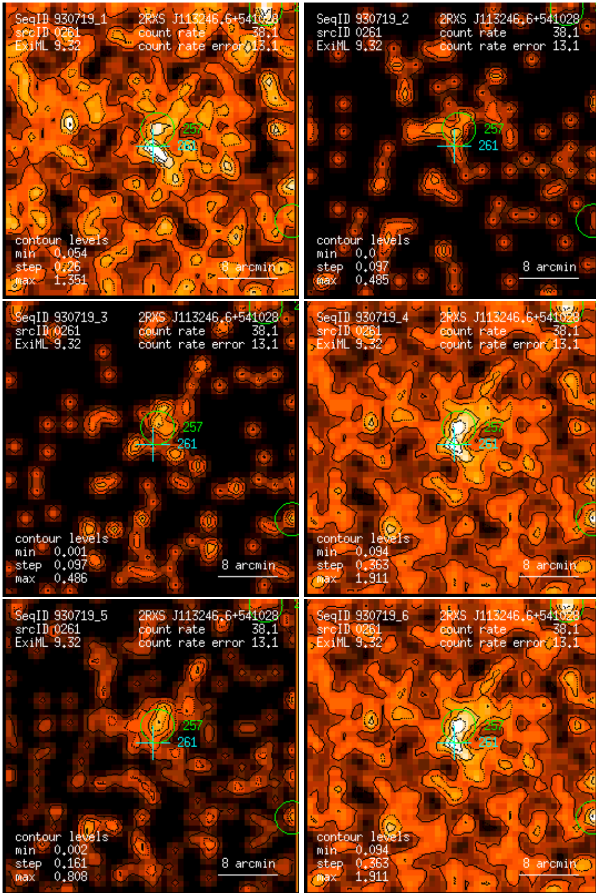
Figure 261: RASS 930719: detection 0261: band rate images, Gaussian filter: (1) PSPC channels 11 – 41, (2) 52 – 90, (3) 91 – 201, (4) 11 – 235, (5) 52 – 201, (6) 11 – 201. Broad band rates in counts/ks. Band rate contour levels in counts/ks/arcmin 2 .
