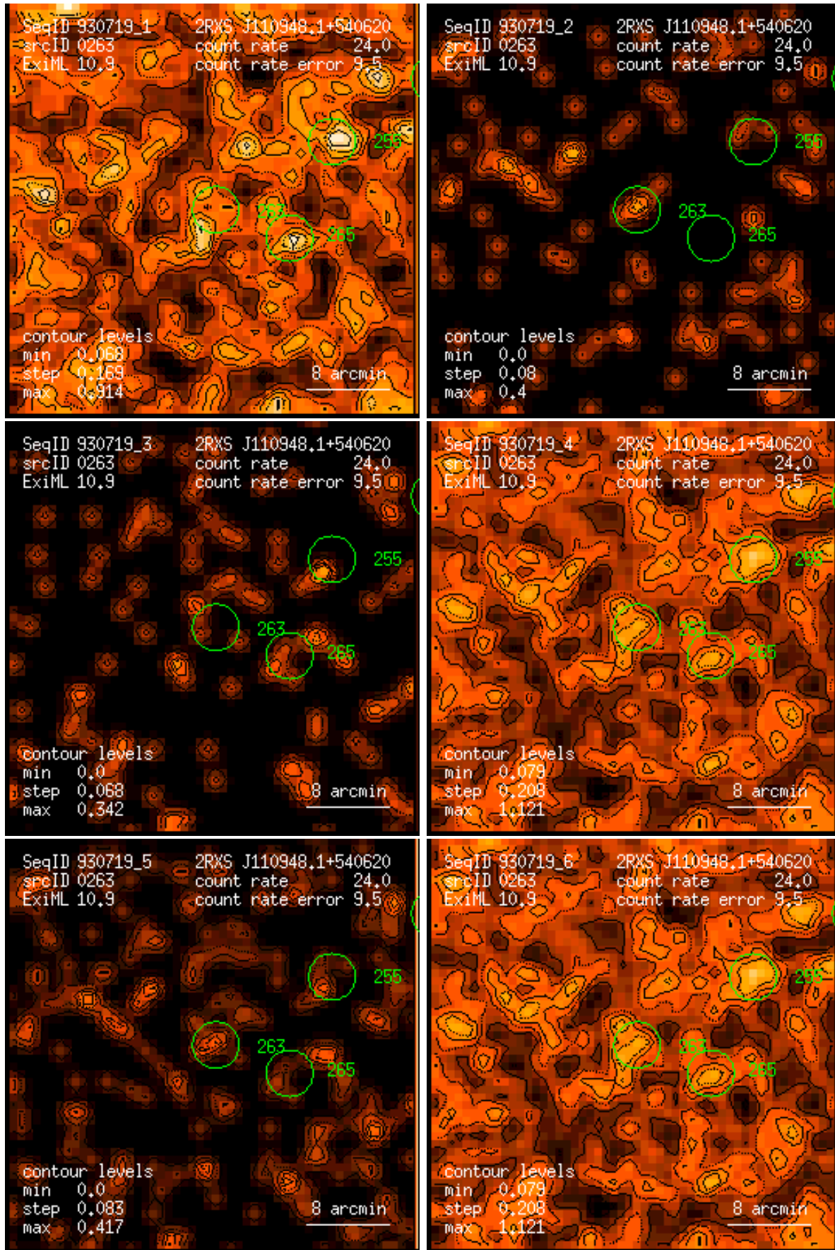
Figure 263: RASS 930719: detection 0263: band rate images, Gaussian filter: (1) PSPC channels 11 – 41, (2) 52 – 90, (3) 91 – 201, (4) 11 – 235, (5) 52 – 201, (6) 11 – 201. Broad band rates in counts/ks. Band rate contour levels in counts/ks/arcmin 2 .
