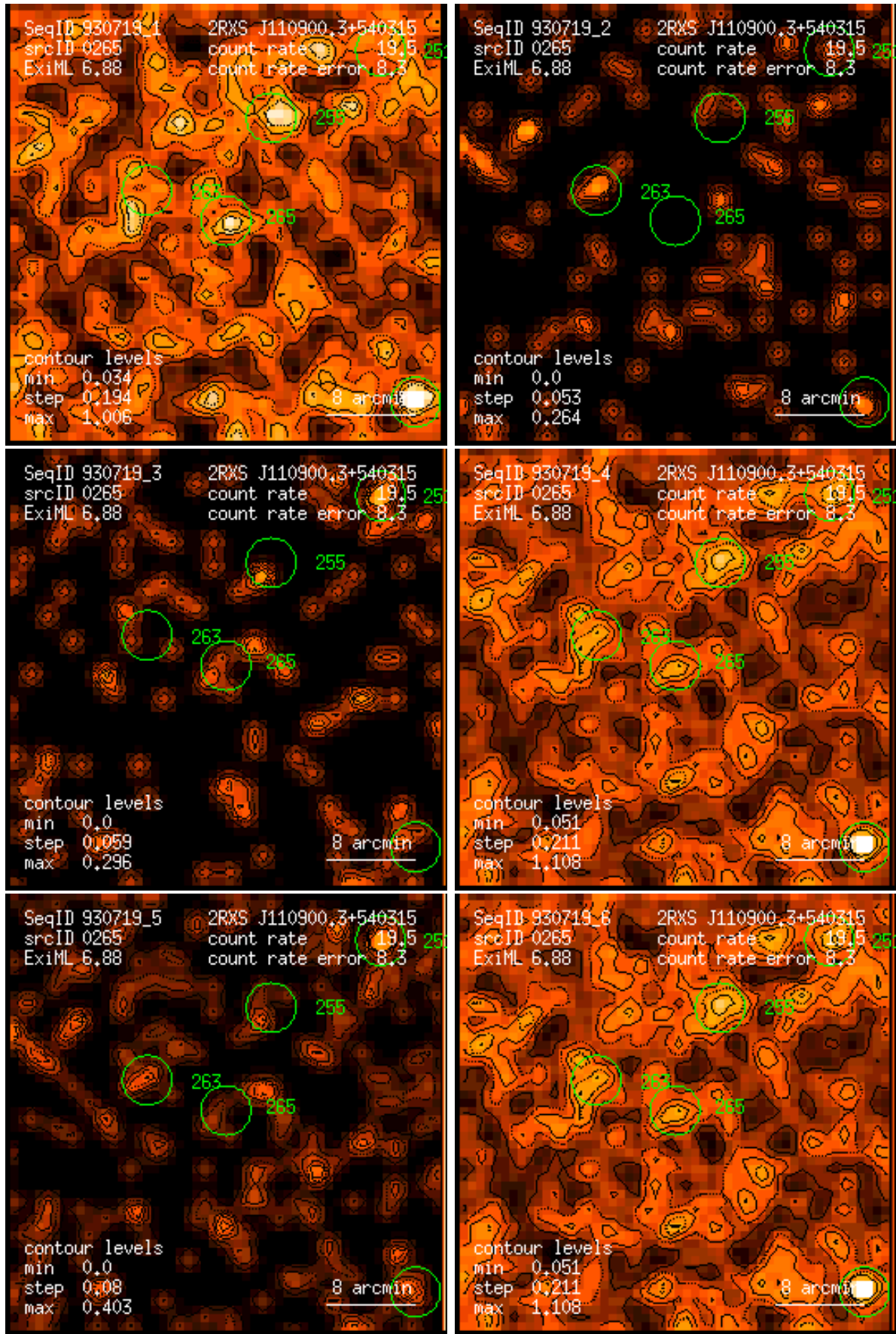
Figure 265: RASS 930719: detection 0265: band rate images, Gaussian filter: (1) PSPC channels 11 – 41, (2) 52 – 90, (3) 91 – 201, (4) 11 – 235, (5) 52 – 201, (6) 11 – 201. Broad band rates in counts/ks. Band rate contour levels in counts/ks/arcmin 2 .
