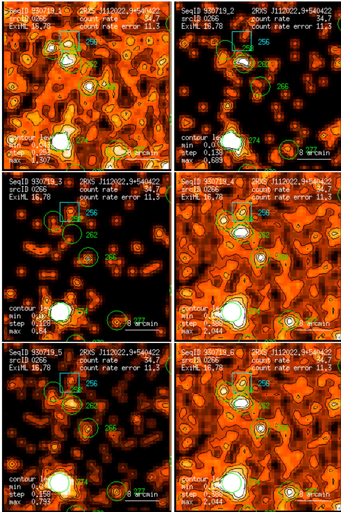
Figure 266: RASS 930719: detection 0266: band rate images, Gaussian filter: (1) PSPC channels 11 – 41, (2) 52 – 90, (3) 91 – 201, (4) 11 – 235, (5) 52 – 201, (6) 11 – 201. Broad band rates in counts/ks. Band rate contour levels in counts/ks/arcmin 2 .
