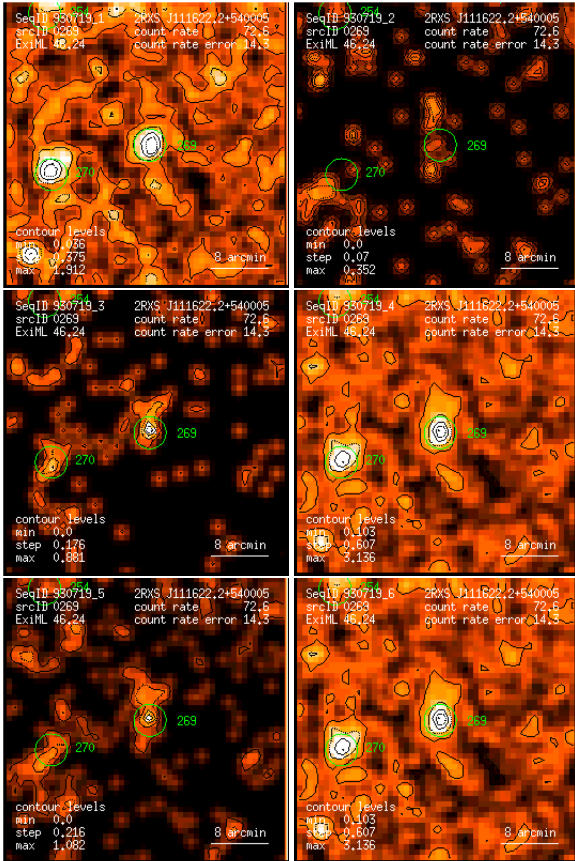
Figure 269: RASS 930719: detection 0269: band rate images, Gaussian filter: (1) PSPC channels 11 – 41, (2) 52 – 90, (3) 91 – 201, (4) 11 – 235, (5) 52 – 201, (6) 11 – 201. Broad band rates in counts/ks. Band rate contour levels in counts/ks/arcmin 2 .
