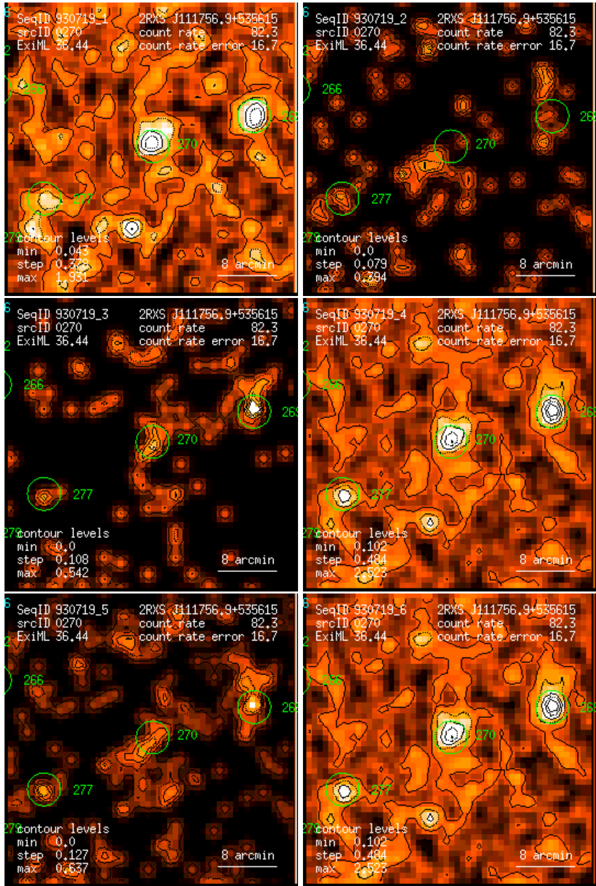
Figure 270: RASS 930719: detection 0270: band rate images, Gaussian filter: (1) PSPC channels 11 – 41, (2) 52 – 90, (3) 91 – 201, (4) 11 – 235, (5) 52 – 201, (6) 11 – 201. Broad band rates in counts/ks. Band rate contour levels in counts/ks/arcmin 2 .
