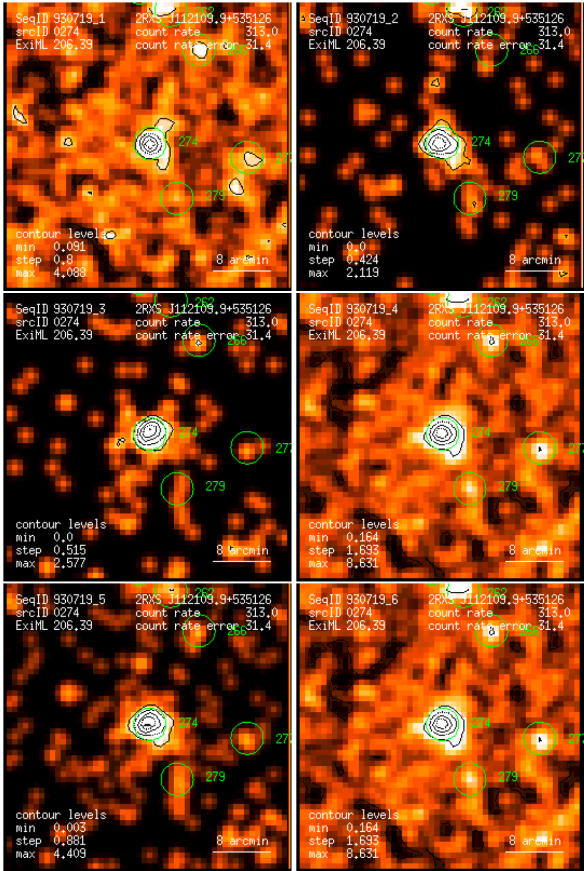
Figure 274: RASS 930719: detection 0274: band rate images, Gaussian filter: (1) PSPC channels 11 – 41, (2) 52 – 90, (3) 91 – 201, (4) 11 – 235, (5) 52 – 201, (6) 11 – 201. Broad band rates in counts/ks. Band rate contour levels in counts/ks/arcmin 2 .
