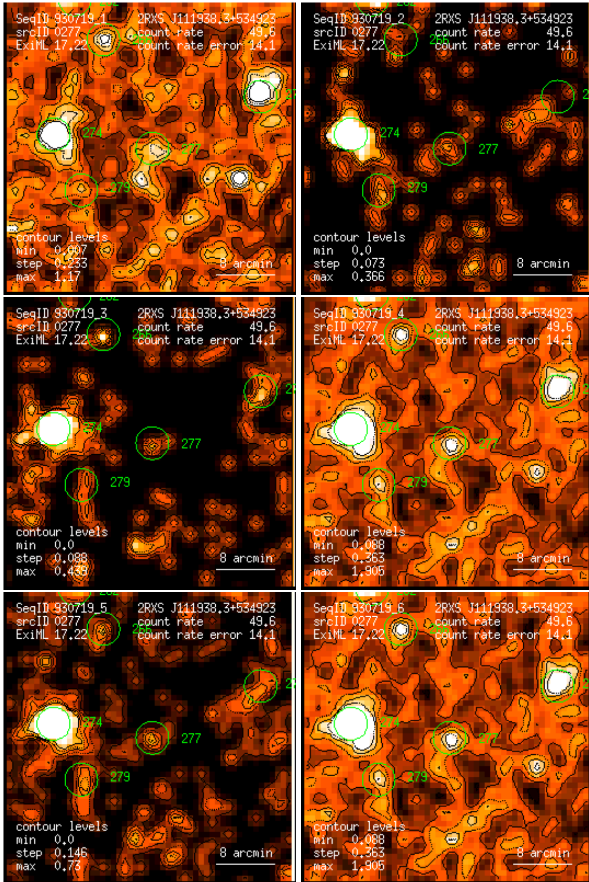
Figure 277: RASS 930719: detection 0277: band rate images, Gaussian filter: (1) PSPC channels 11 – 41, (2) 52 – 90, (3) 91 – 201, (4) 11 – 235, (5) 52 – 201, (6) 11 – 201. Broad band rates in counts/ks. Band rate contour levels in counts/ks/arcmin 2 .
