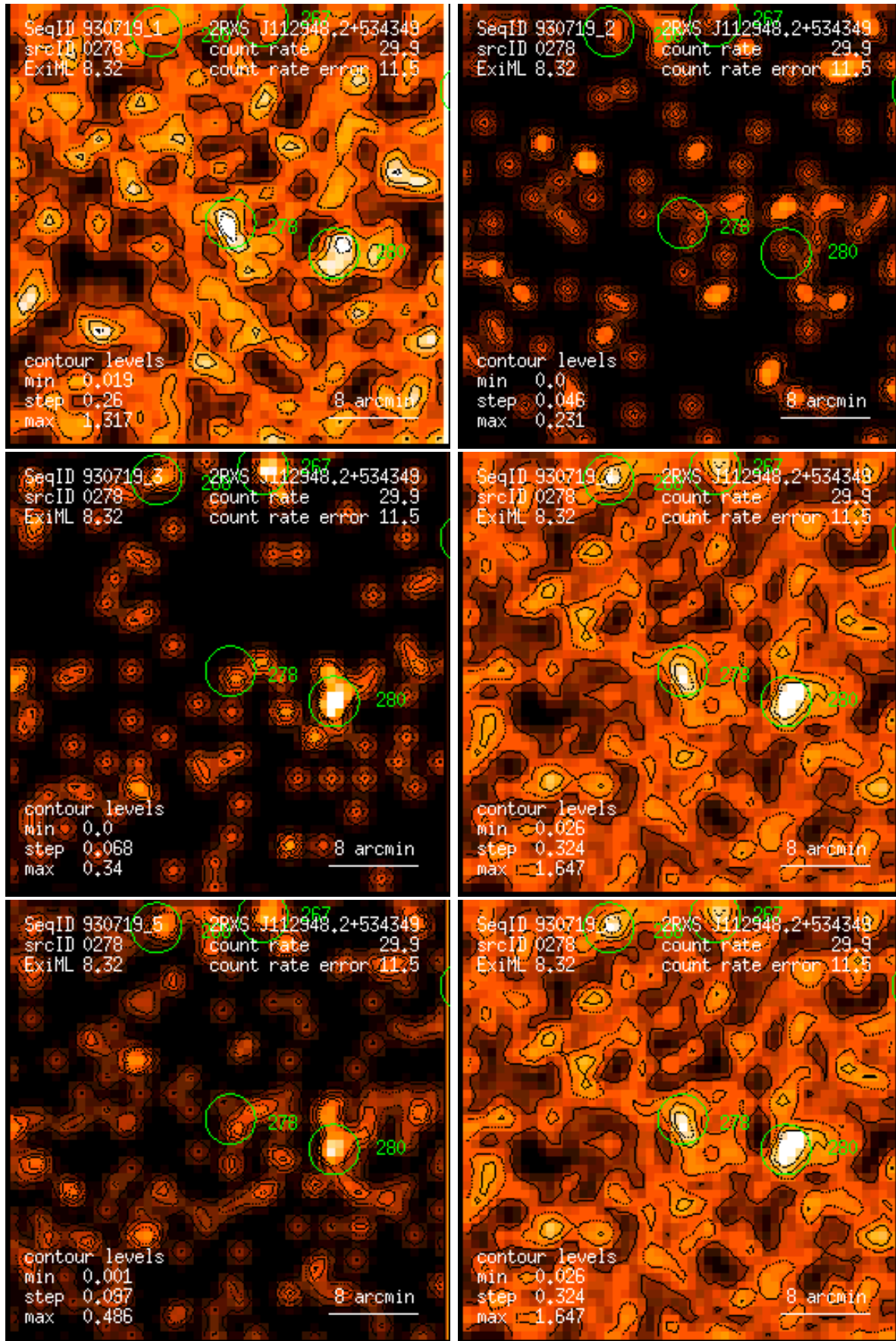
Figure 278: RASS 930719: detection 0278: band rate images, Gaussian filter: (1) PSPC channels 11 – 41, (2) 52 – 90, (3) 91 – 201, (4) 11 – 235, (5) 52 – 201, (6) 11 – 201. Broad band rates in counts/ks. Band rate contour levels in counts/ks/arcmin 2 .
