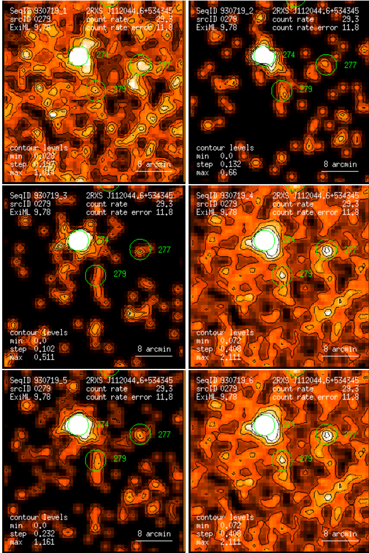
Figure 279: RASS 930719: detection 0279: band rate images, Gaussian filter: (1) PSPC channels 11 – 41, (2) 52 – 90, (3) 91 – 201, (4) 11 – 235, (5) 52 – 201, (6) 11 – 201. Broad band rates in counts/ks. Band rate contour levels in counts/ks/arcmin 2 .
