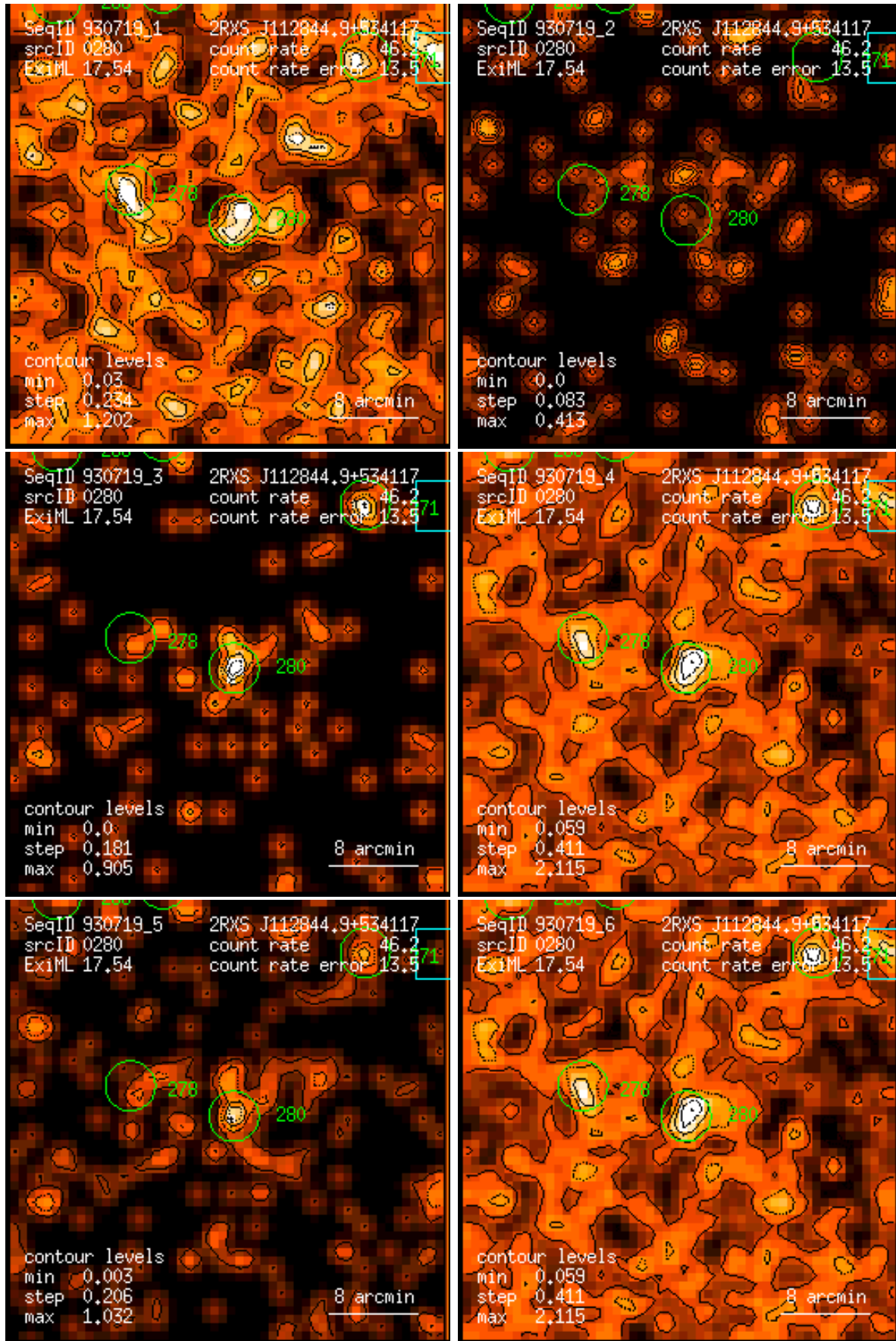
Figure 280: RASS 930719: detection 0280: band rate images, Gaussian filter: (1) PSPC channels 11 – 41, (2) 52 – 90, (3) 91 – 201, (4) 11 – 235, (5) 52 – 201, (6) 11 – 201. Broad band rates in counts/ks. Band rate contour levels in counts/ks/arcmin 2 .
