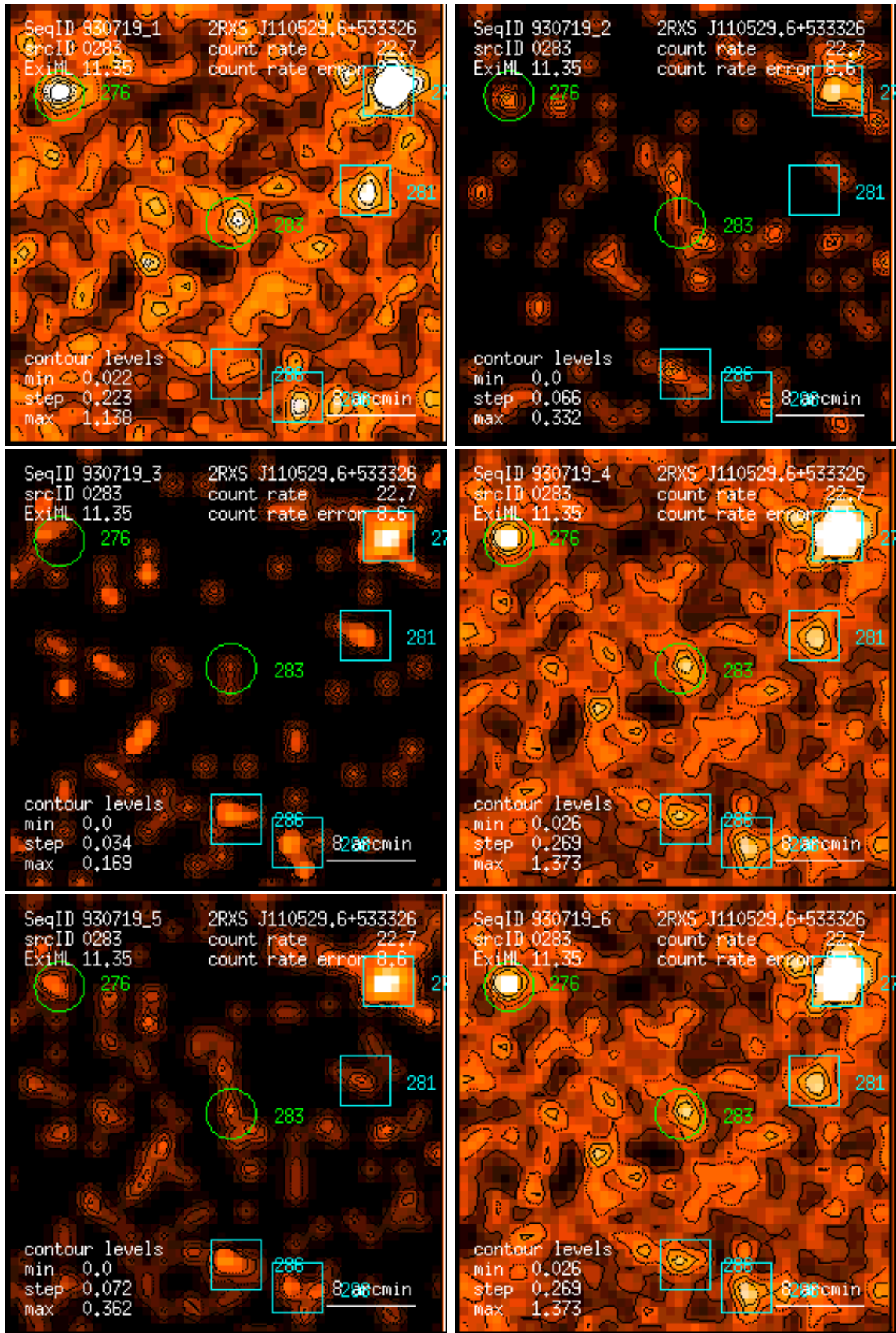
Figure 283: RASS 930719: detection 0283: band rate images, Gaussian filter: (1) PSPC channels 11 – 41, (2) 52 – 90, (3) 91 – 201, (4) 11 – 235, (5) 52 – 201, (6) 11 – 201. Broad band rates in counts/ks. Band rate contour levels in counts/ks/arcmin 2 .
