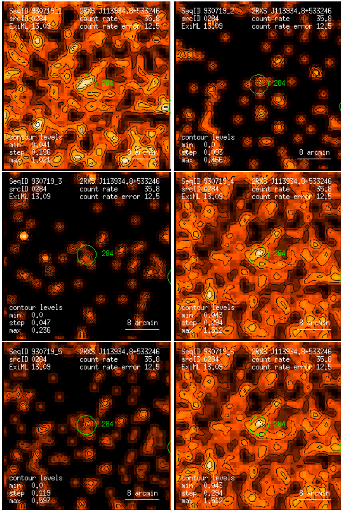
Figure 284: RASS 930719: detection 0284: band rate images, Gaussian filter: (1) PSPC channels 11 – 41, (2) 52 – 90, (3) 91 – 201, (4) 11 – 235, (5) 52 – 201, (6) 11 – 201. Broad band rates in counts/ks. Band rate contour levels in counts/ks/arcmin 2 .
