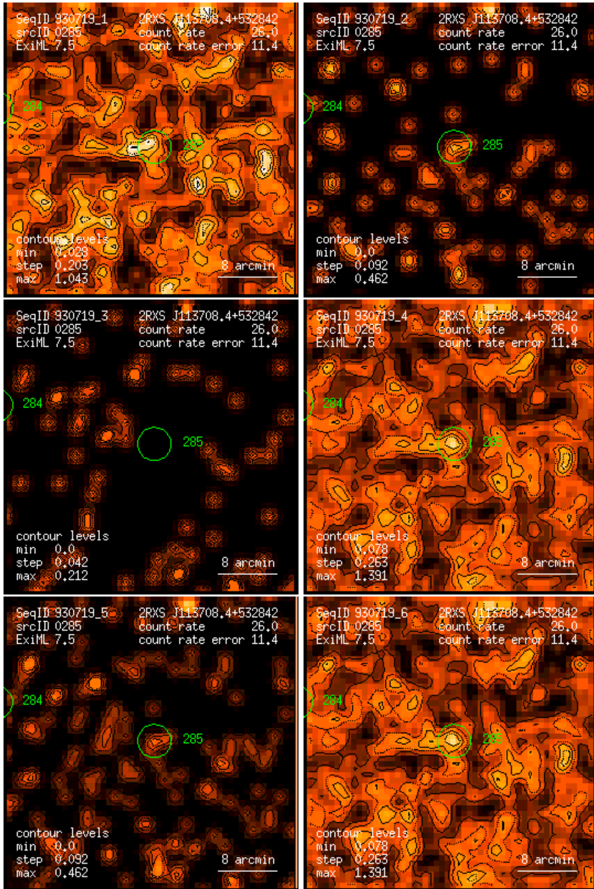
Figure 285: RASS 930719: detection 0285: band rate images, Gaussian filter: (1) PSPC channels 11 – 41, (2) 52 – 90, (3) 91 – 201, (4) 11 – 235, (5) 52 – 201, (6) 11 – 201. Broad band rates in counts/ks. Band rate contour levels in counts/ks/arcmin 2 .
