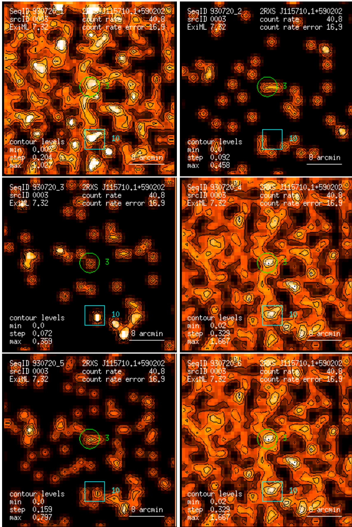
Figure 3: RASS 930720: detection 0003: band rate images, Gaussian filter: (1) PSPC channels 11 – 41, (2) 52 – 90, (3) 91 – 201, (4) 11 – 235, (5) 52 – 201, (6) 11 – 201. Broad band rates in counts/ks. Band rate contour levels in counts/ks/arcmin 2 .
