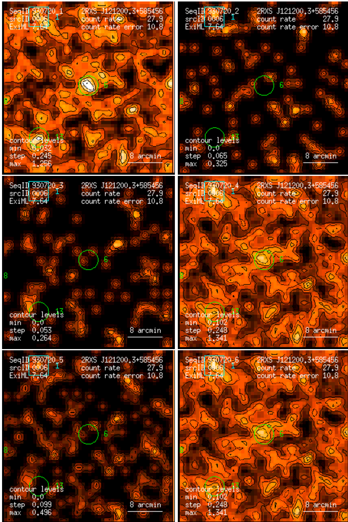
Figure 6: RASS 930720: detection 0006: band rate images, Gaussian filter: (1) PSPC channels 11 – 41, (2) 52 – 90, (3) 91 – 201, (4) 11 – 235, (5) 52 – 201, (6) 11 – 201. Broad band rates in counts/ks. Band rate contour levels in counts/ks/arcmin 2 .
