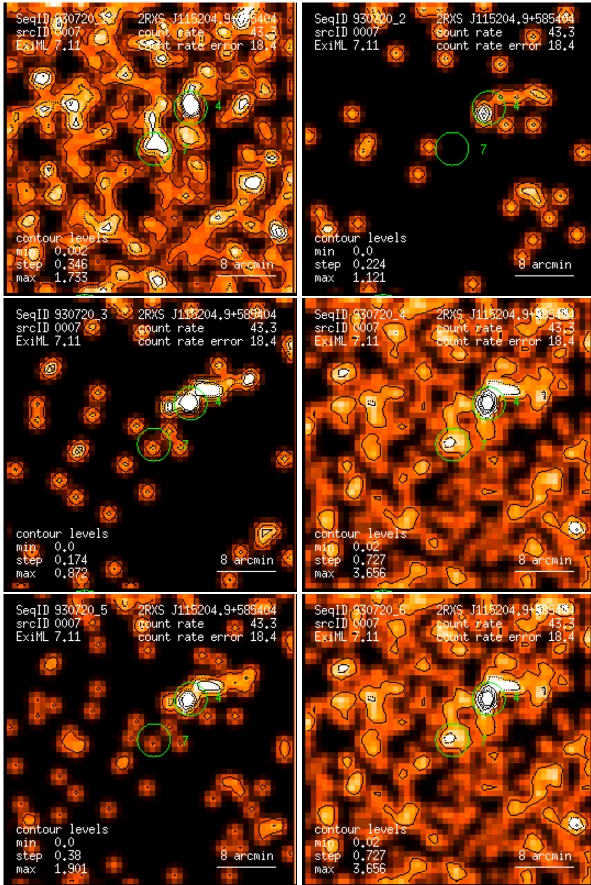
Figure 7: RASS 930720: detection 0007: band rate images, Gaussian filter: (1) PSPC channels 11 – 41, (2) 52 – 90, (3) 91 – 201, (4) 11 – 235, (5) 52 – 201, (6) 11 – 201. Broad band rates in counts/ks. Band rate contour levels in counts/ks/arcmin 2 .
