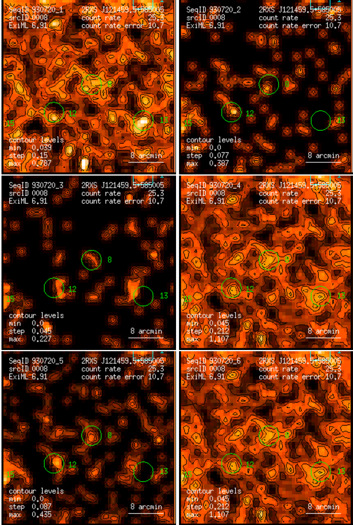
Figure 8: RASS 930720: detection 0008: band rate images, Gaussian filter: (1) PSPC channels 11 – 41, (2) 52 – 90, (3) 91 – 201, (4) 11 – 235, (5) 52 – 201, (6) 11 – 201. Broad band rates in counts/ks. Band rate contour levels in counts/ks/arcmin 2 .
