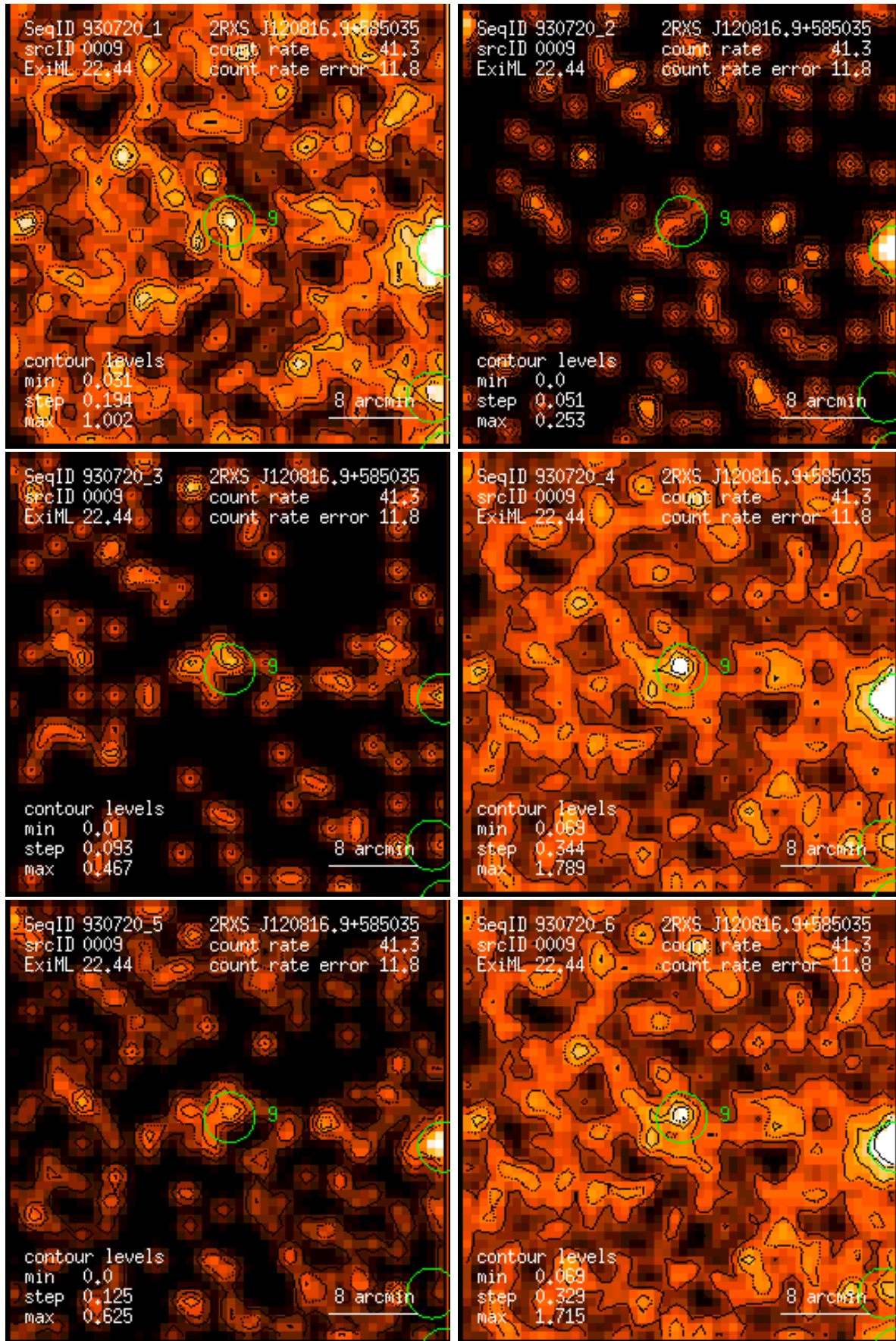
Figure 9: RASS 930720: detection 0009: band rate images, Gaussian filter: (1) PSPC channels 11 – 41, (2) 52 – 90, (3) 91 – 201, (4) 11 – 235, (5) 52 – 201, (6) 11 – 201. Broad band rates in counts/ks. Band rate contour levels in counts/ks/arcmin 2 .
