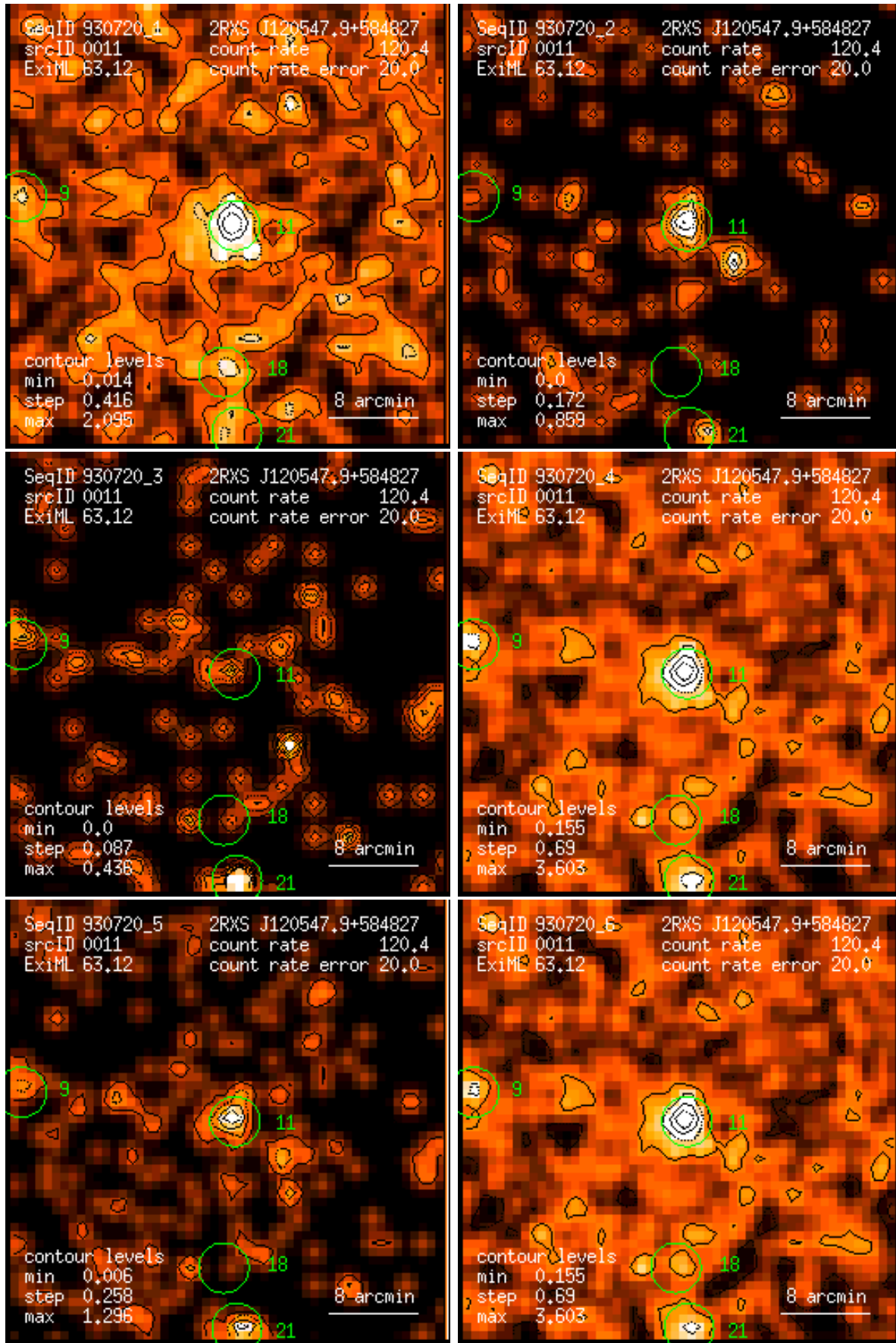
Figure 11: RASS 930720: detection 0011: band rate images, Gaussian filter: (1) PSPC channels 11 – 41, (2) 52 – 90, (3) 91 – 201, (4) 11 – 235, (5) 52 – 201, (6) 11 – 201. Broad band rates in counts/ks. Band rate contour levels in counts/ks/arcmin 2 .
