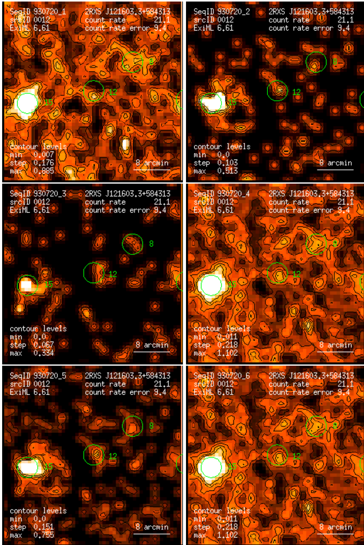
Figure 12: RASS 930720: detection 0012: band rate images, Gaussian filter: (1) PSPC channels 11 – 41, (2) 52 – 90, (3) 91 – 201, (4) 11 – 235, (5) 52 – 201, (6) 11 – 201. Broad band rates in counts/ks. Band rate contour levels in counts/ks/arcmin 2 .
