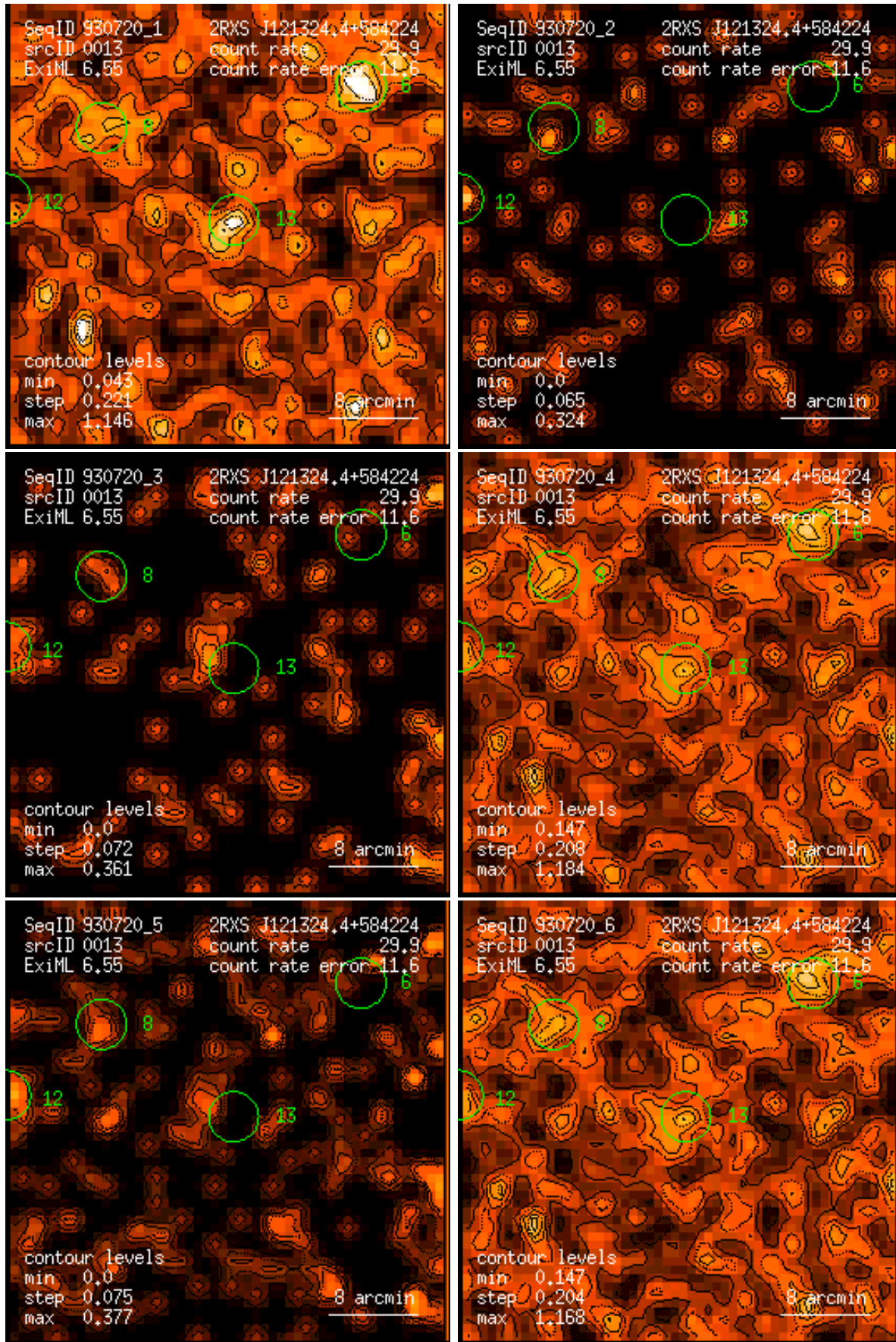
Figure 13: RASS 930720: detection 0013: band rate images, Gaussian filter: (1) PSPC channels 11 – 41, (2) 52 – 90, (3) 91 – 201, (4) 11 – 235, (5) 52 – 201, (6) 11 – 201. Broad band rates in counts/ks. Band rate contour levels in counts/ks/arcmin 2 .
