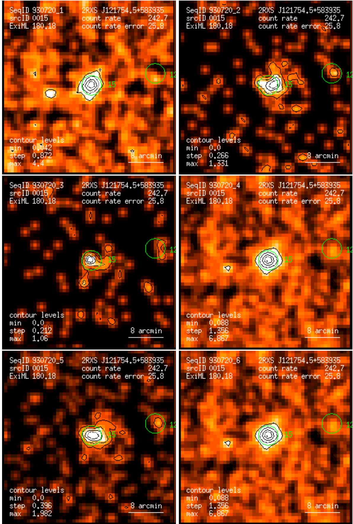
Figure 15: RASS 930720: detection 0015: band rate images, Gaussian filter: (1) PSPC channels 11 – 41, (2) 52 – 90, (3) 91 – 201, (4) 11 – 235, (5) 52 – 201, (6) 11 – 201. Broad band rates in counts/ks. Band rate contour levels in counts/ks/arcmin 2 .
