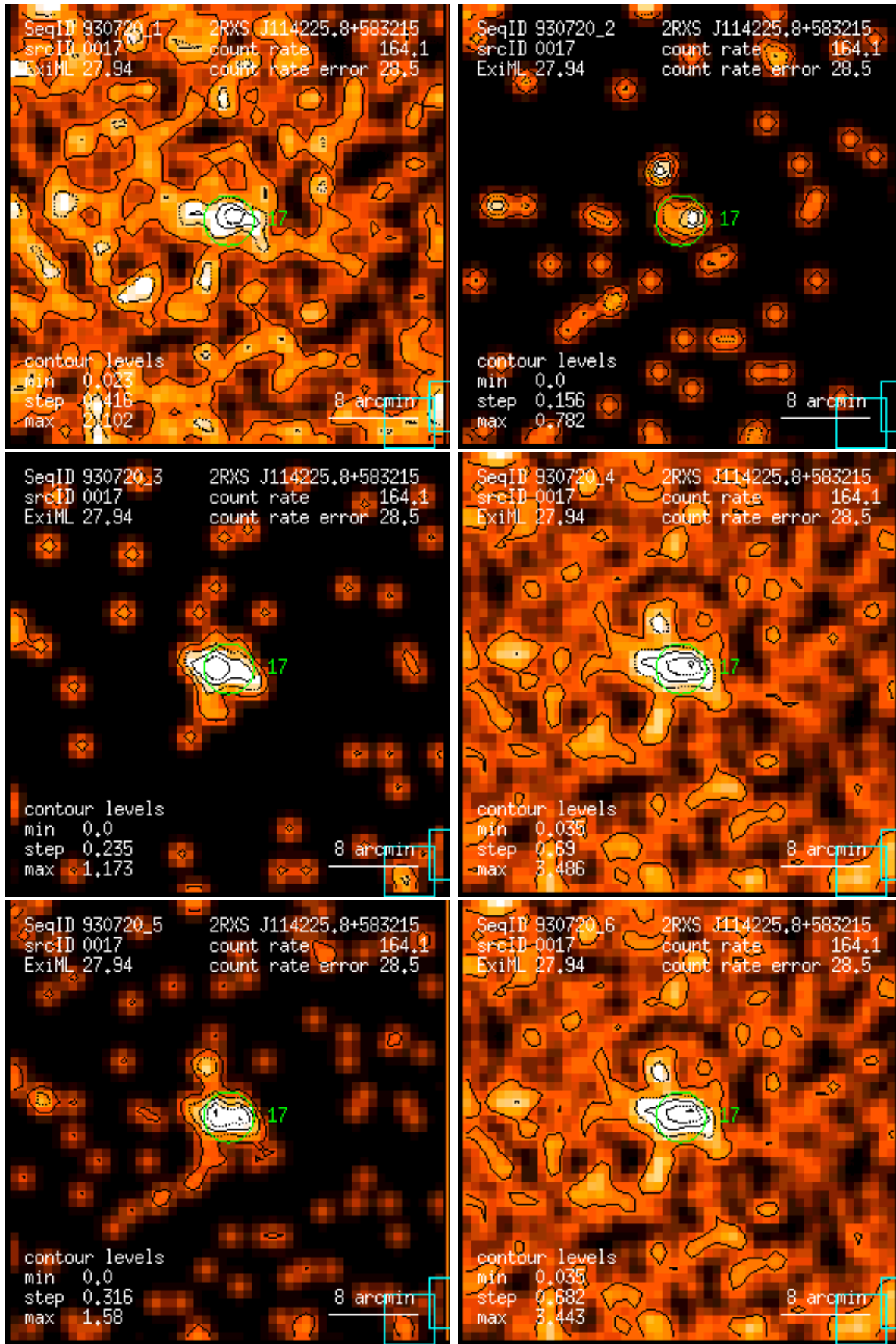
Figure 17: RASS 930720: detection 0017: band rate images, Gaussian filter: (1) PSPC channels 11 – 41, (2) 52 – 90, (3) 91 – 201, (4) 11 – 235, (5) 52 – 201, (6) 11 – 201. Broad band rates in counts/ks. Band rate contour levels in counts/ks/arcmin 2 .
