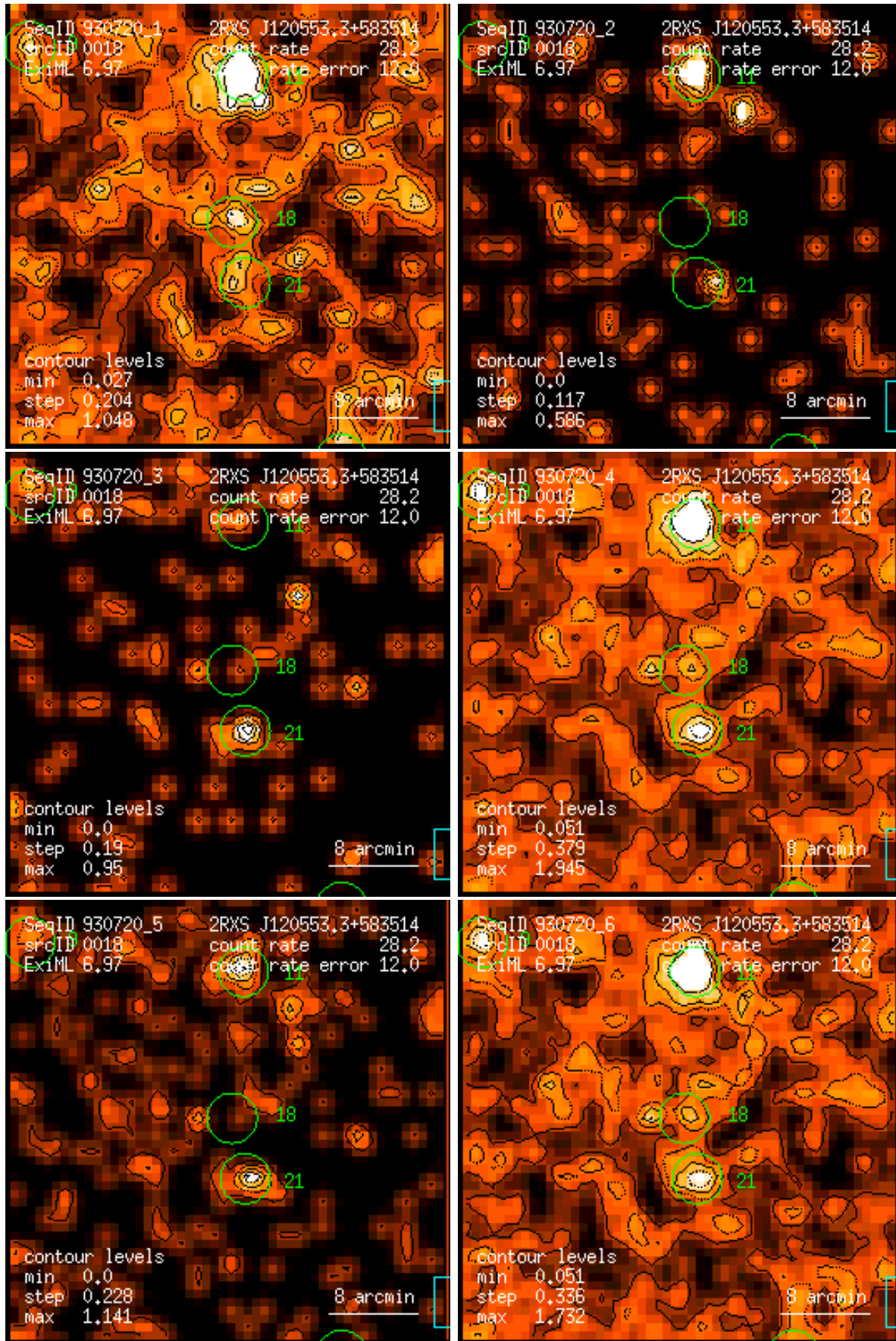
Figure 18: RASS 930720: detection 0018: band rate images, Gaussian filter: (1) PSPC channels 11 – 41, (2) 52 – 90, (3) 91 – 201, (4) 11 – 235, (5) 52 – 201, (6) 11 – 201. Broad band rates in counts/ks. Band rate contour levels in counts/ks/arcmin 2 .
