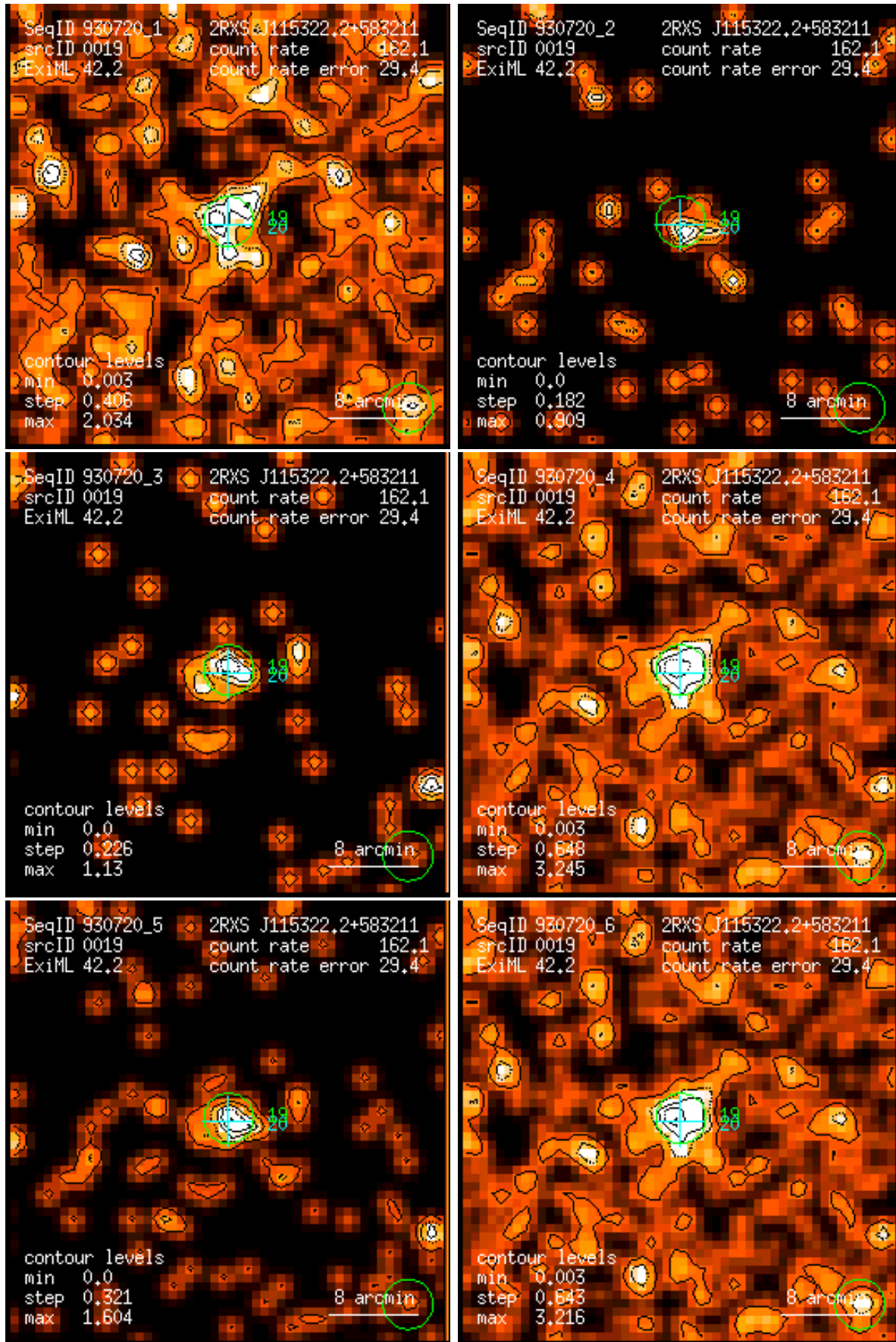
Figure 19: RASS 930720: detection 0019: band rate images, Gaussian filter: (1) PSPC channels 11 – 41, (2) 52 – 90, (3) 91 – 201, (4) 11 – 235, (5) 52 – 201, (6) 11 – 201. Broad band rates in counts/ks. Band rate contour levels in counts/ks/arcmin 2 .
