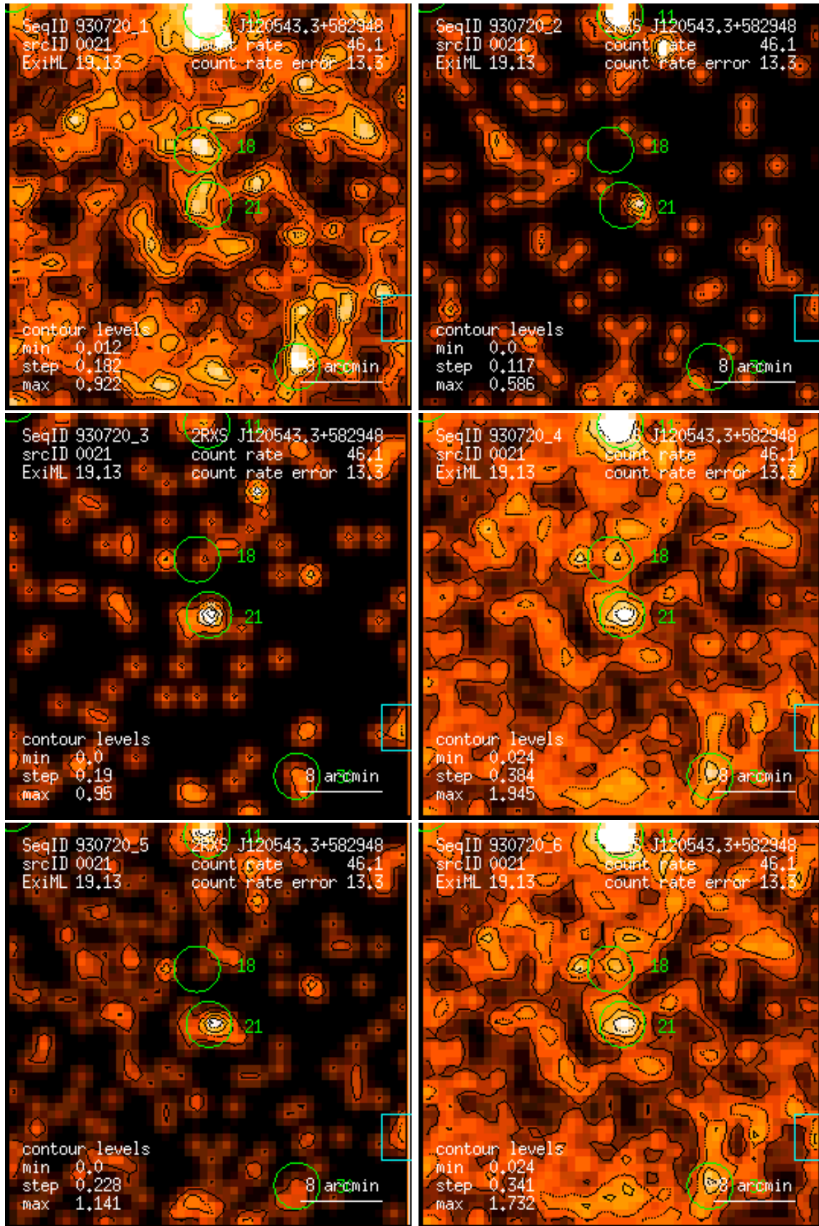
Figure 21: RASS 930720: detection 0021: band rate images, Gaussian filter: (1) PSPC channels 11 – 41, (2) 52 – 90, (3) 91 – 201, (4) 11 – 235, (5) 52 – 201, (6) 11 – 201. Broad band rates in counts/ks. Band rate contour levels in counts/ks/arcmin 2 .
