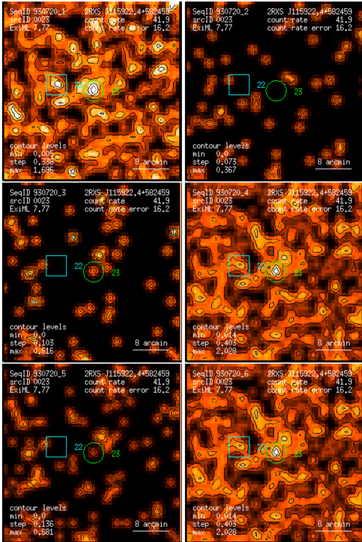
Figure 23: RASS 930720: detection 0023: band rate images, Gaussian filter: (1) PSPC channels 11 – 41, (2) 52 – 90, (3) 91 – 201, (4) 11 – 235, (5) 52 – 201, (6) 11 – 201. Broad band rates in counts/ks. Band rate contour levels in counts/ks/arcmin 2 .
