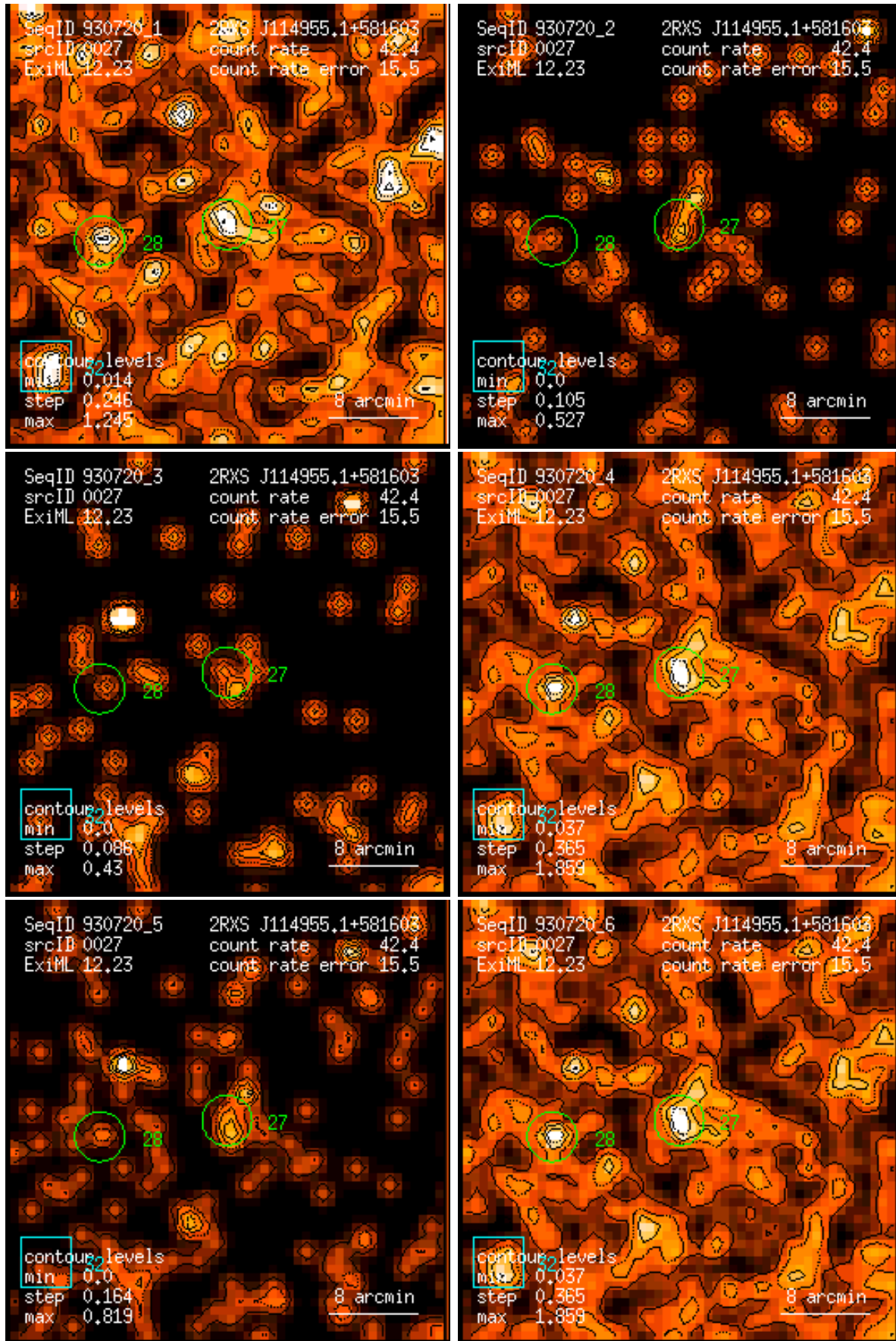
Figure 27: RASS 930720: detection 0027: band rate images, Gaussian filter: (1) PSPC channels 11 – 41, (2) 52 – 90, (3) 91 – 201, (4) 11 – 235, (5) 52 – 201, (6) 11 – 201. Broad band rates in counts/ks. Band rate contour levels in counts/ks/arcmin 2 .
