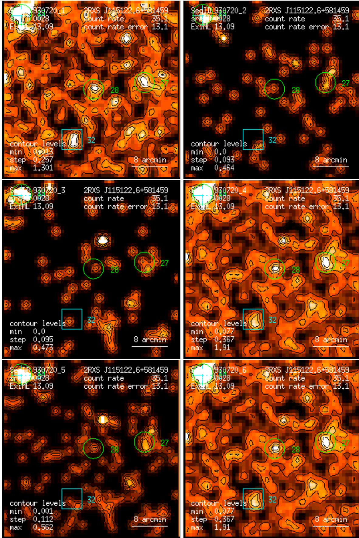
Figure 28: RASS 930720: detection 0028: band rate images, Gaussian filter: (1) PSPC channels 11 – 41, (2) 52 – 90, (3) 91 – 201, (4) 11 – 235, (5) 52 – 201, (6) 11 – 201. Broad band rates in counts/ks. Band rate contour levels in counts/ks/arcmin 2 .
