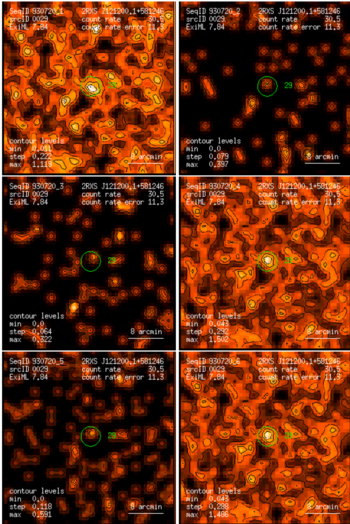
Figure 29: RASS 930720: detection 0029: band rate images, Gaussian filter: (1) PSPC channels 11 – 41, (2) 52 – 90, (3) 91 – 201, (4) 11 – 235, (5) 52 – 201, (6) 11 – 201. Broad band rates in counts/ks. Band rate contour levels in counts/ks/arcmin 2 .
