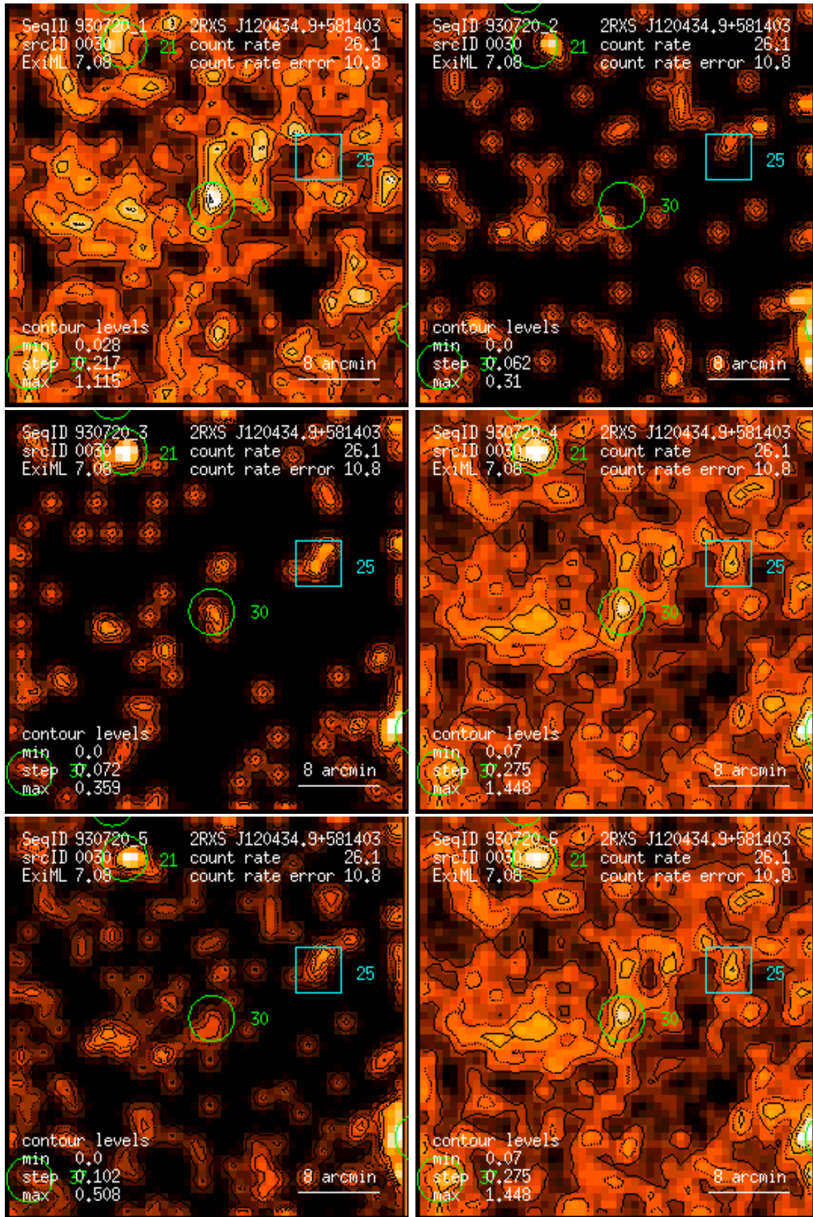
Figure 30: RASS 930720: detection 0030: band rate images, Gaussian filter: (1) PSPC channels 11 – 41, (2) 52 – 90, (3) 91 – 201, (4) 11 – 235, (5) 52 – 201, (6) 11 – 201. Broad band rates in counts/ks. Band rate contour levels in counts/ks/arcmin 2 .
