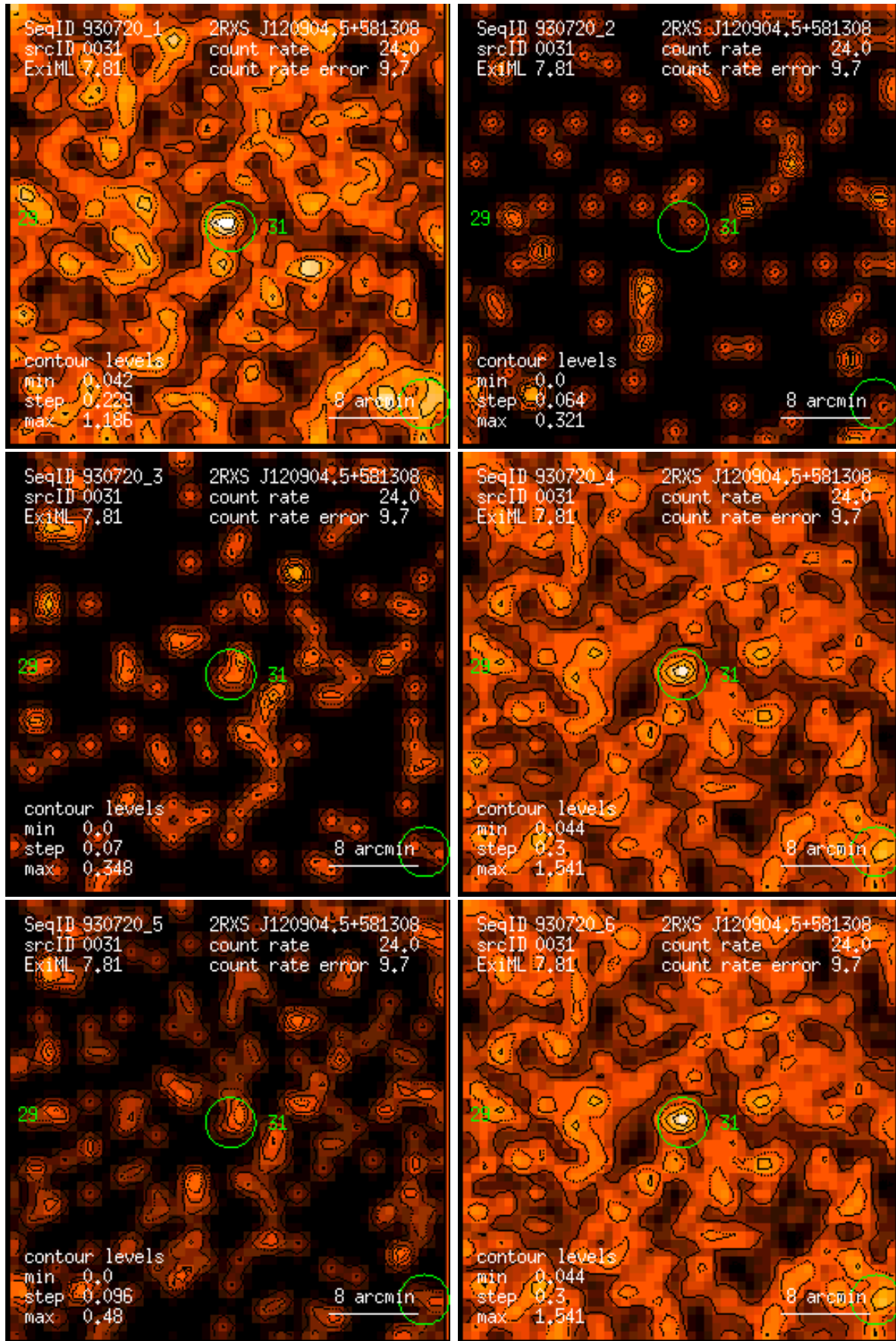
Figure 31: RASS 930720: detection 0031: band rate images, Gaussian filter: (1) PSPC channels 11 – 41, (2) 52 – 90, (3) 91 – 201, (4) 11 – 235, (5) 52 – 201, (6) 11 – 201. Broad band rates in counts/ks. Band rate contour levels in counts/ks/arcmin 2 .
