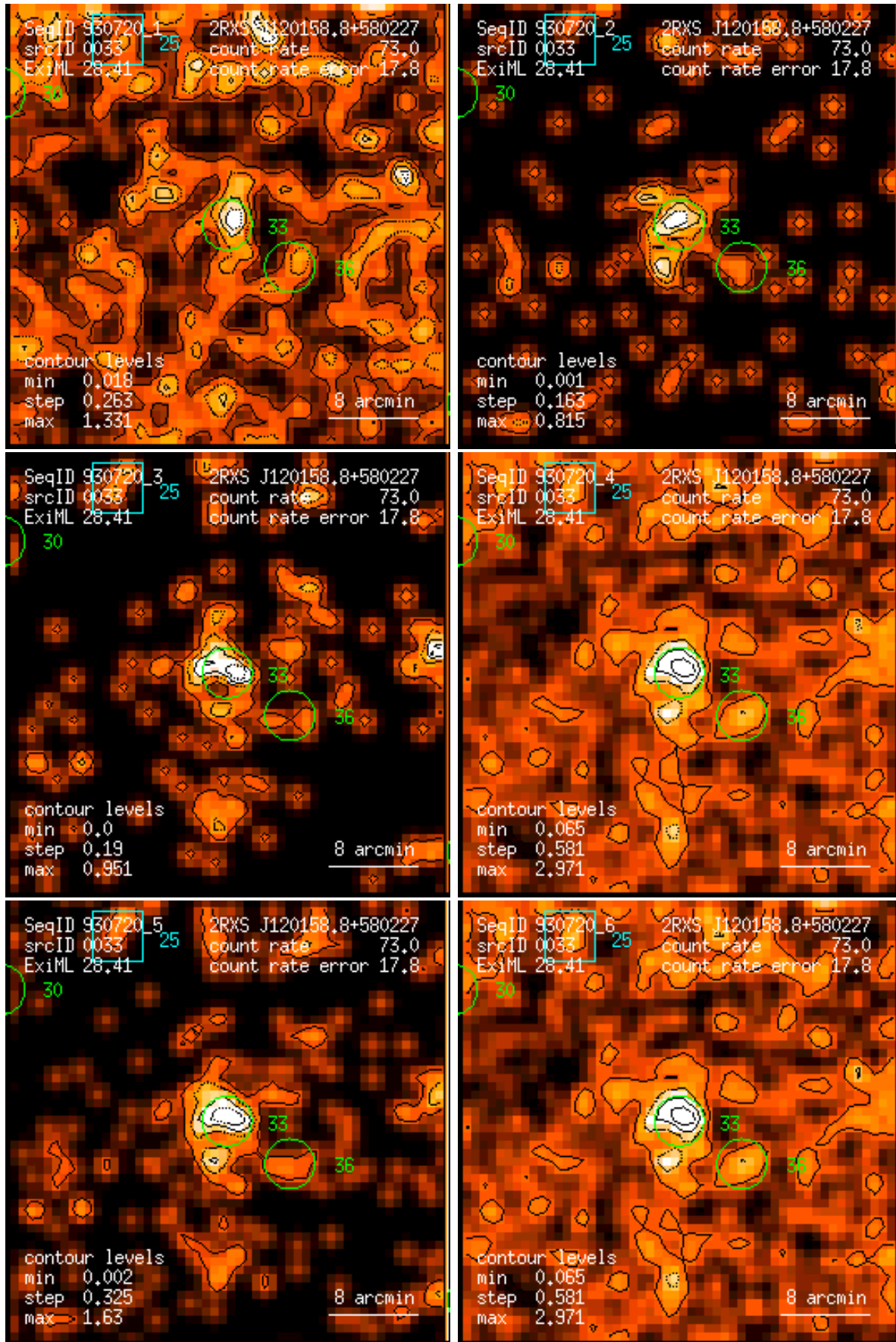
Figure 33: RASS 930720: detection 0033: band rate images, Gaussian filter: (1) PSPC channels 11 – 41, (2) 52 – 90, (3) 91 – 201, (4) 11 – 235, (5) 52 – 201, (6) 11 – 201. Broad band rates in counts/ks. Band rate contour levels in counts/ks/arcmin 2 .
